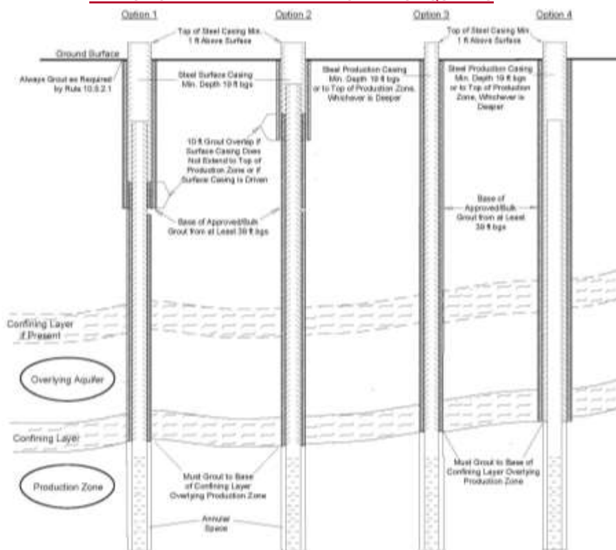
FIGURE 9 LARAMIE-FOX HILLS AQUIFER
