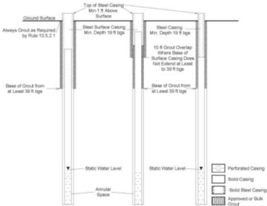
FIGURE 7a TYPE 2 AQUIFER WELLS COMPLETED IN TYPE 2 (UNCONFINED BEDROCK) AQUIFER NOT OVERLAIN BY TYPE 3 AQUIFER
