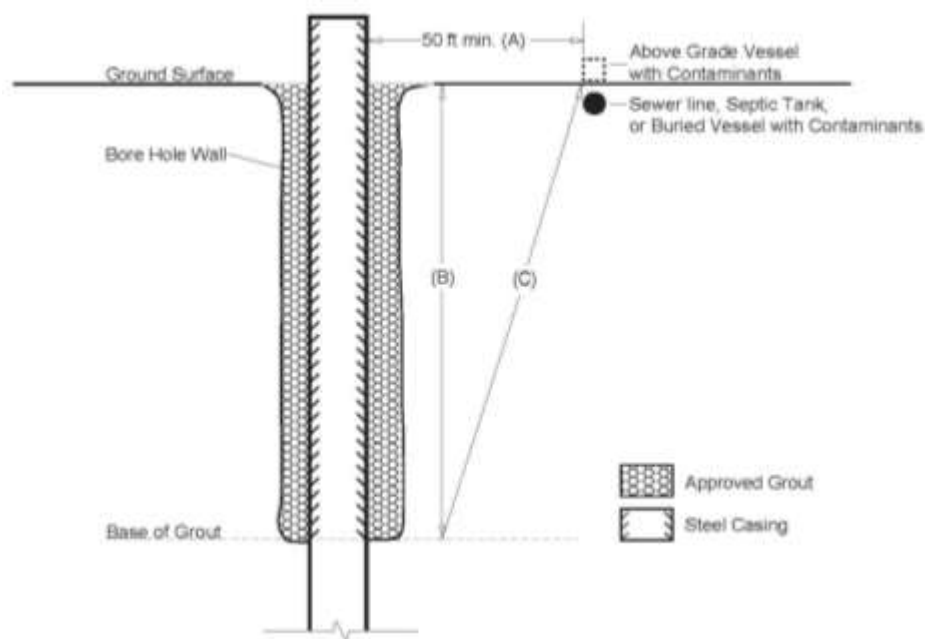
Figure 4b. Schematic of the minimum distance (A) to a well from a sewer line, septic tank, or other above or below ground vessel containing contaminants (Rule 10.2.2). Exceptions to Rule 10.2.2 may be granted through a variance request; if distance A is less than 50 ft., distance C must equal 50 feet or more.
