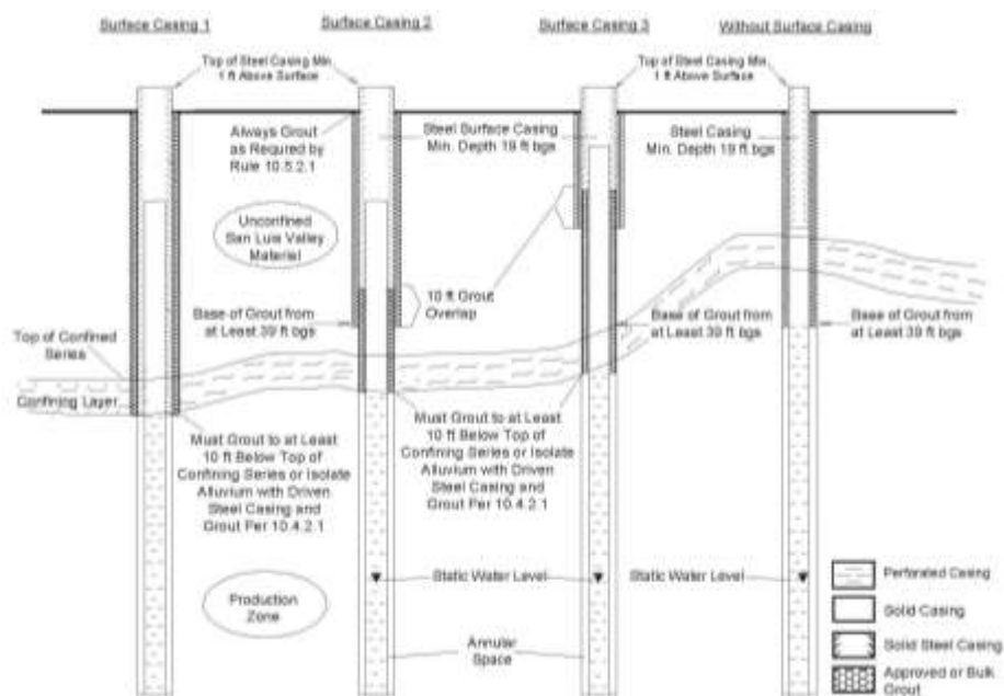
Figure 10. Schematic diagram for wells constructed into the Confined San Luis Valley aquifer
