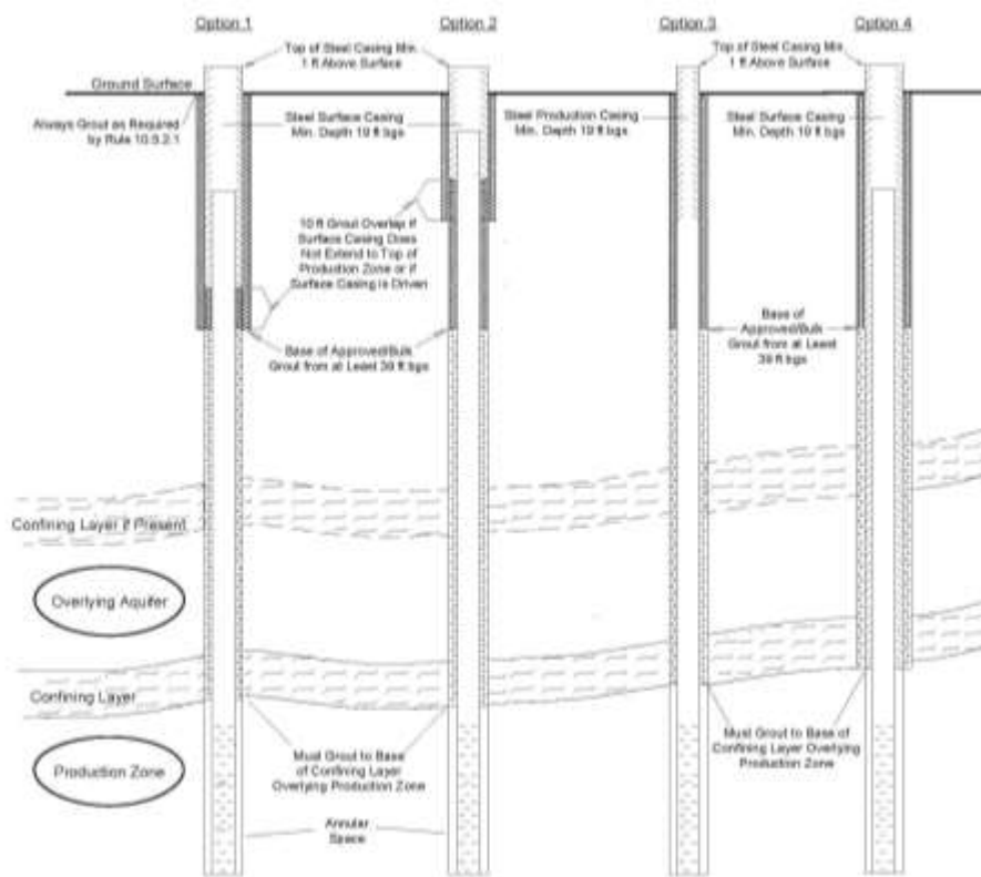
Figure 6. Schematic diagram for wells that penetrate through one or more confining units and are constructed into a Type 1 (confined) aquifer.
