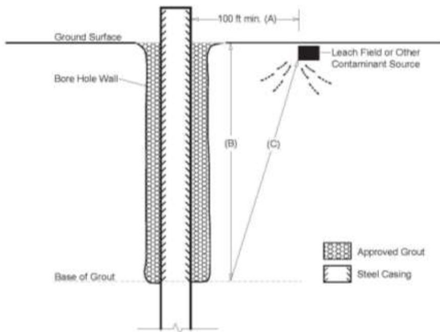
Figure 4a. Schematic of the minimum distance (A) to a well from a leach field or other source of contaminants (Rule 10.2.2). Exceptions to Rule 10.2.2 may be granted through a variance request; if distance A is less than 100 ft., distance C must equal 100 feet or more.
