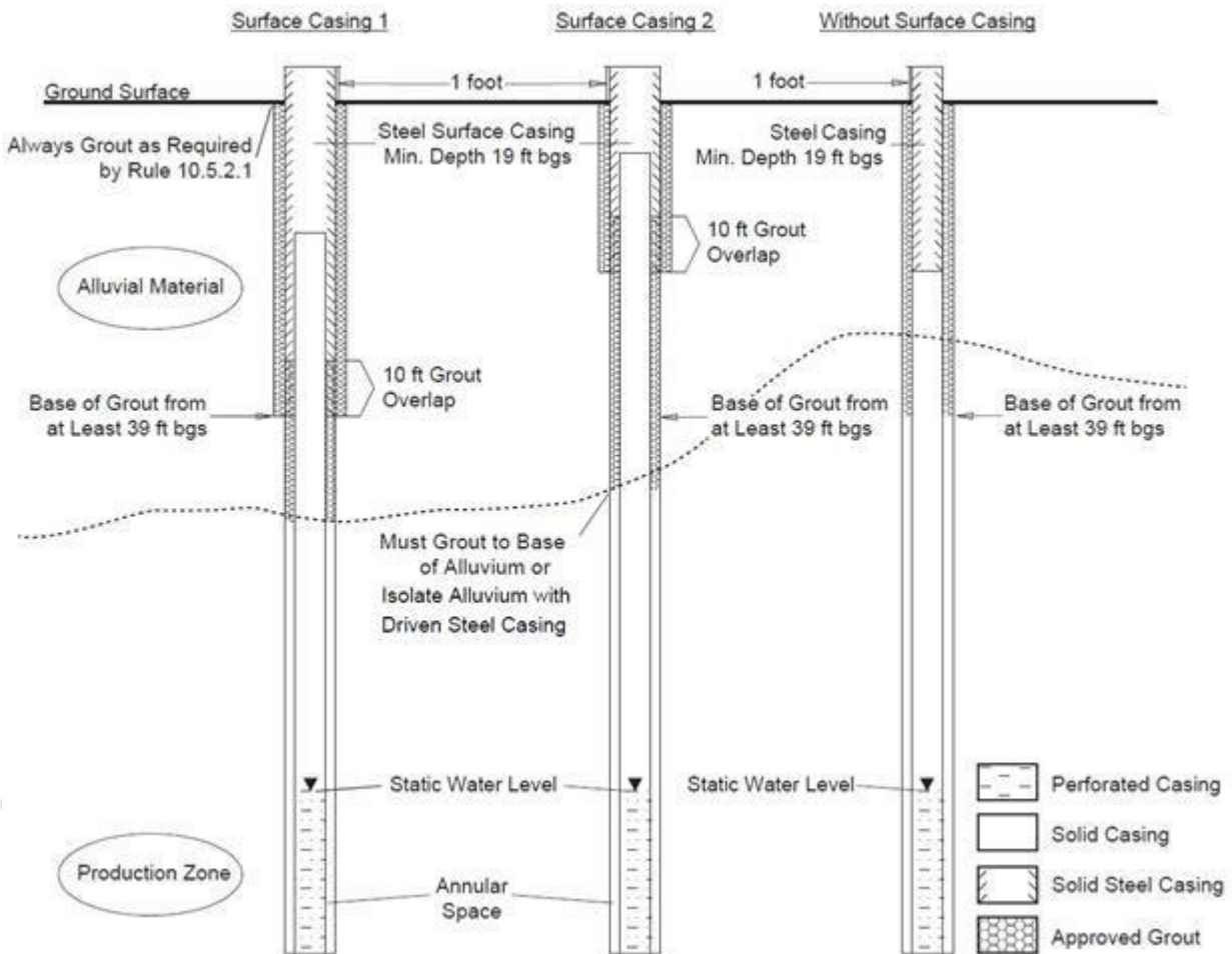
FIGURE 6d TYPE 2 AQUIFER WELLS COMPLETED IN UNCONFINED BEDROCK AQUIFERS (OVERLAIN BY TYPE 3 AQUIFER)
