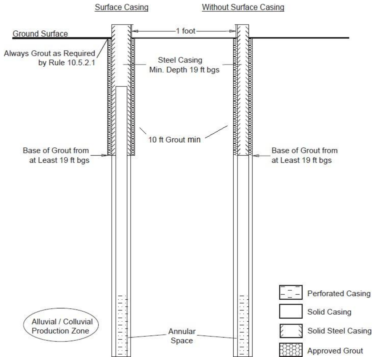
Figure 6e. Schematic diagram for wells constructed into Type 3 (unconsolidated) aquifers.
