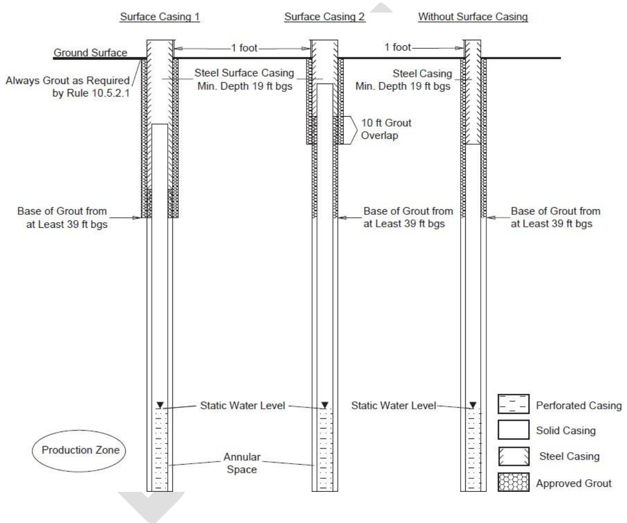
Figure 6c. Schematic diagram for wells constructed into Type 2 (unconfined bedrock) aquifers, not overlain by a Type 3 (unconsolidated) aquifer.
