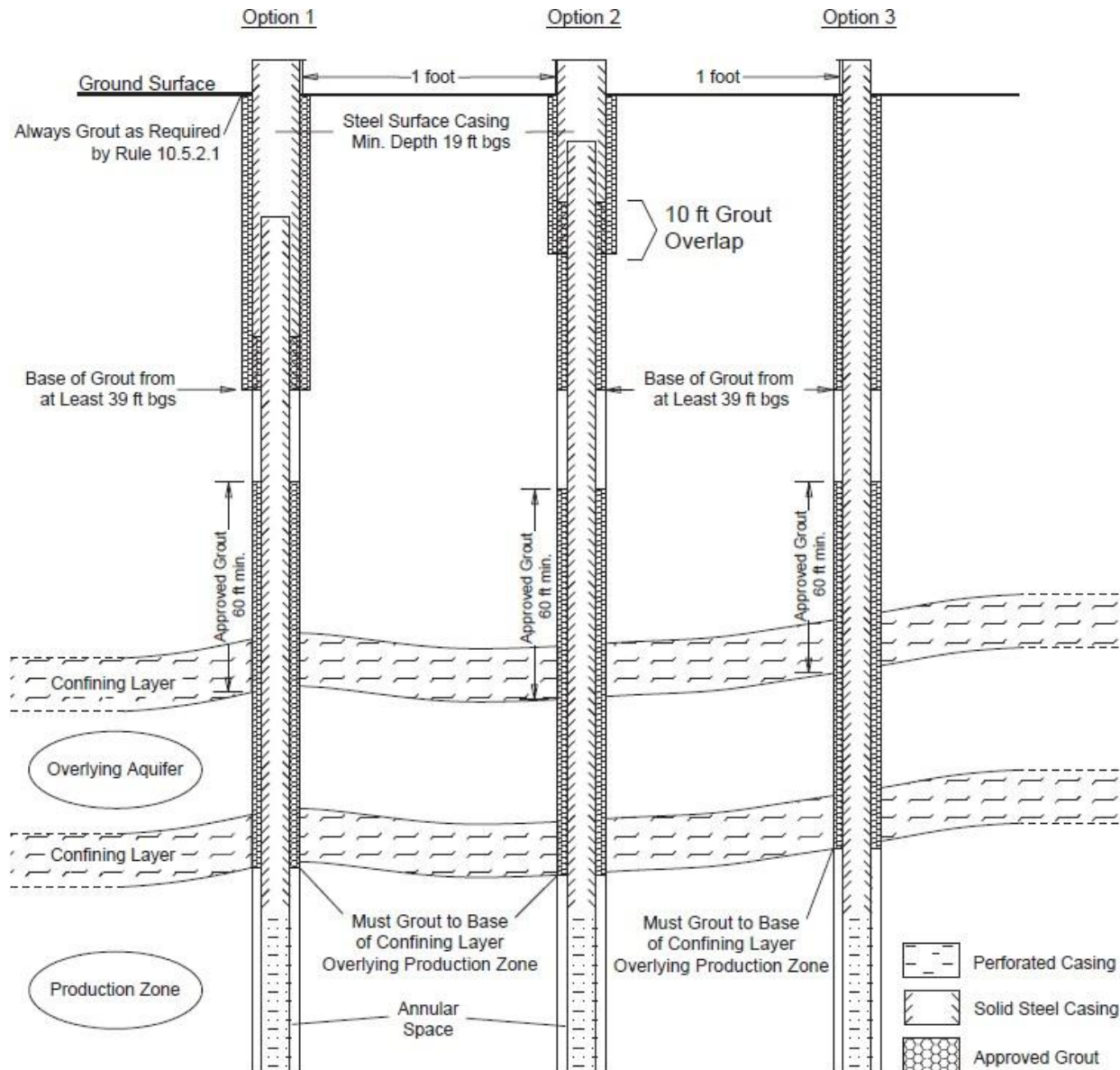
Figure 6b. Schematic diagram for wells that penetrate more than one confining unit and are constructed into a Type I (confined) aquifer.
