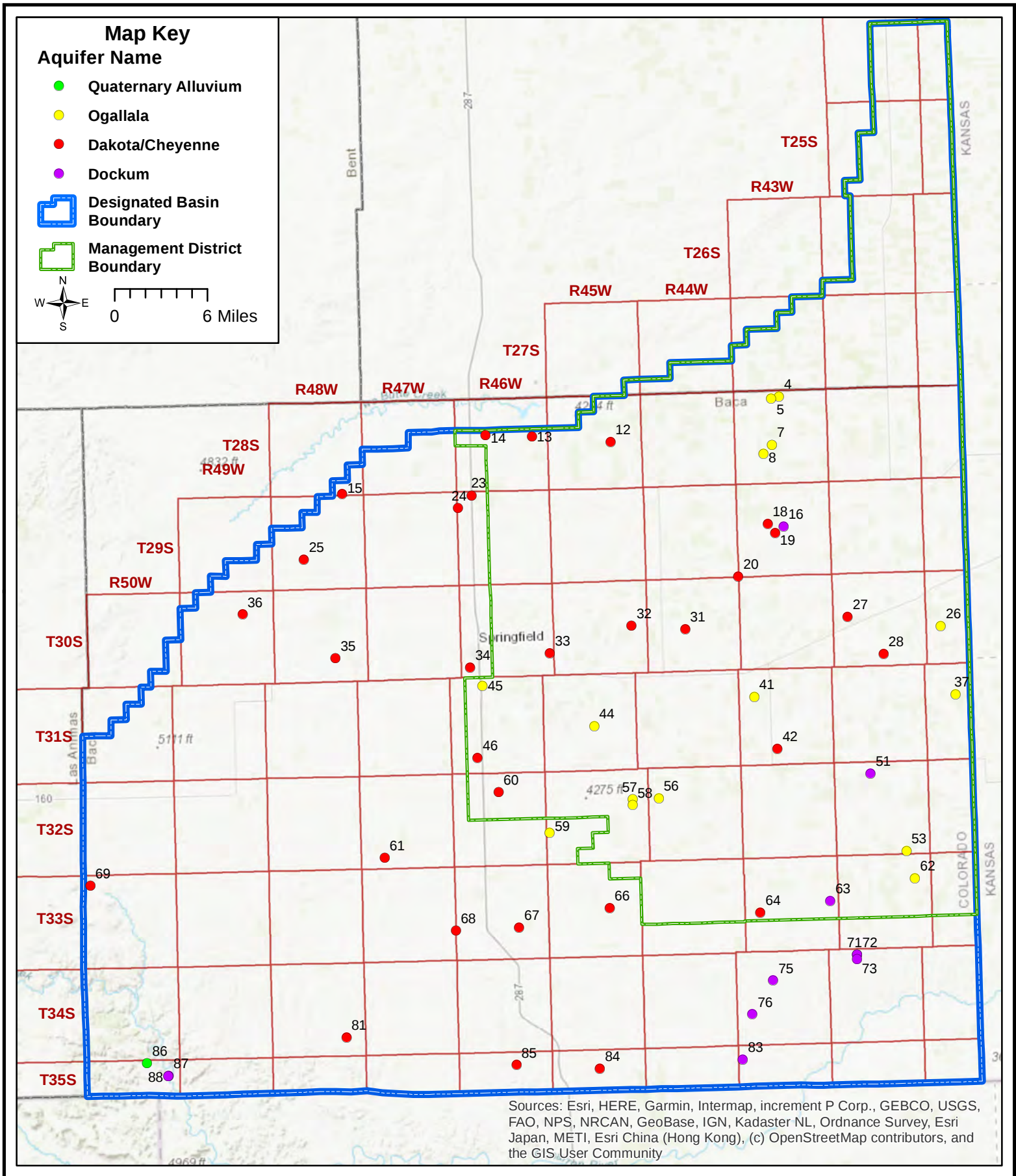
Southern High Plains Designated Basin Aquifers Figure 3
