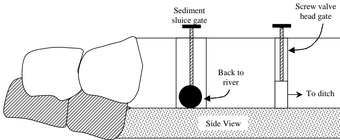
Example of a Cross-Vane/irrigation head gate-sediment sluice
