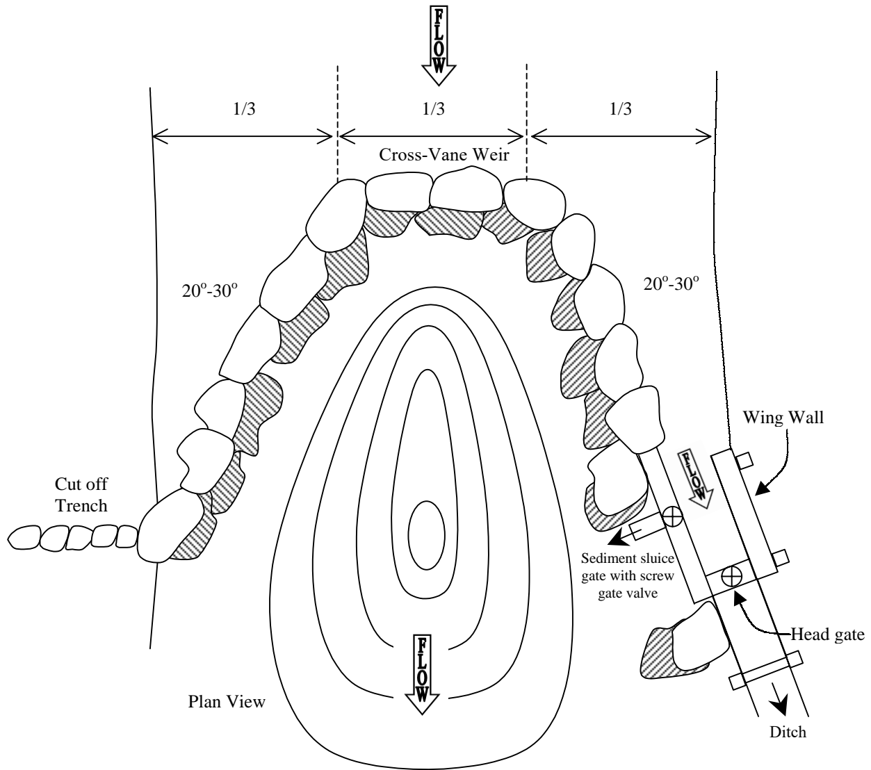
Example of a Cross-Vane/irrigation head gate-sediment sluice
