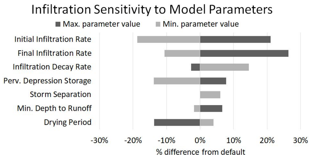
Figure 3.1: Seasonal infiltration response to maximum and minimum WQ-COSM parameter values compared to default or mid-range parameter values. Default or mid-range parameters produce a baseline percent infiltration of 75%.
