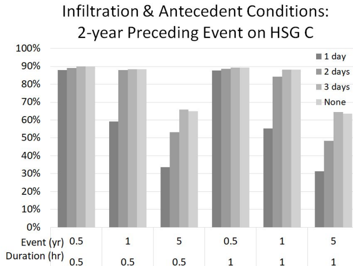
Figure 3.3: The portion of an event that infiltrates decreases when an event occurs shortly after a 2-year event (1 day prior, 2 days prior, etc.).
