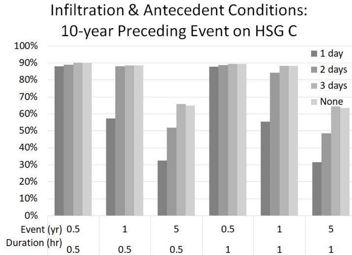
Figure 3.4: The portion of an event that infiltrates decreases when an event occurs shortly after a 10-year event (1 day prior, 2 days prior, etc.).
