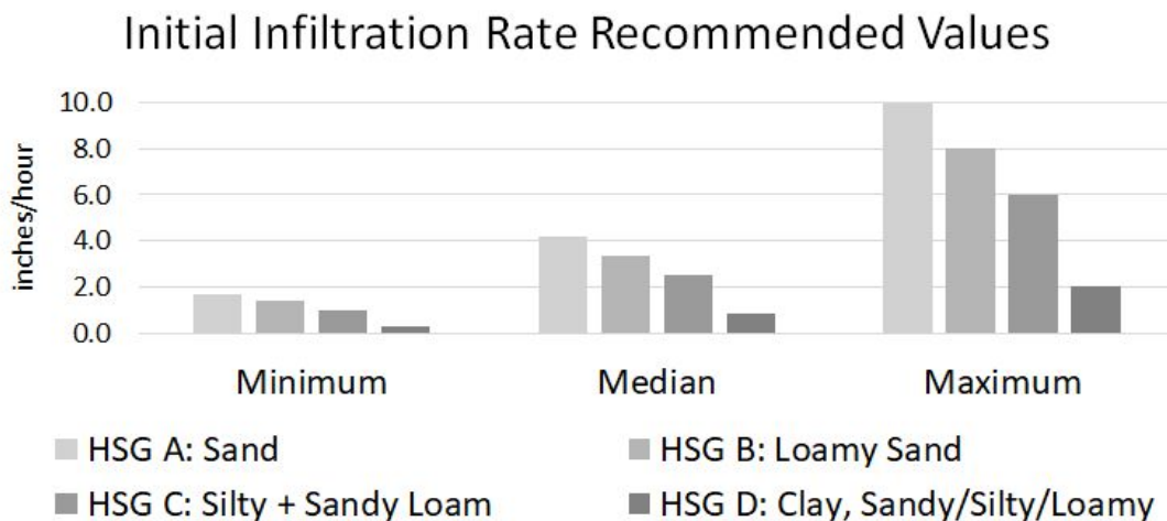
Figure 3.2: Range of recommended initial infiltration rate from WQ-COSM manual
