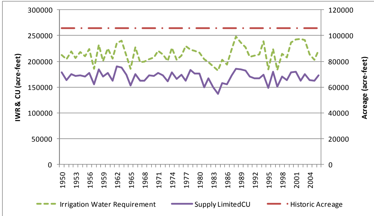
Figure 2 Historic Acreage, Irrigation Water Requirement and Supply Limited CU 1950 through 2006
