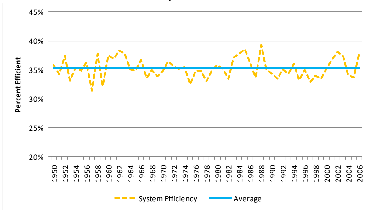
Figure 10 Annual System Efficiencies
