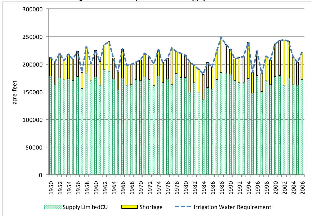
Figure 8 Irrigation Water Requirement and Supply Limited CU
