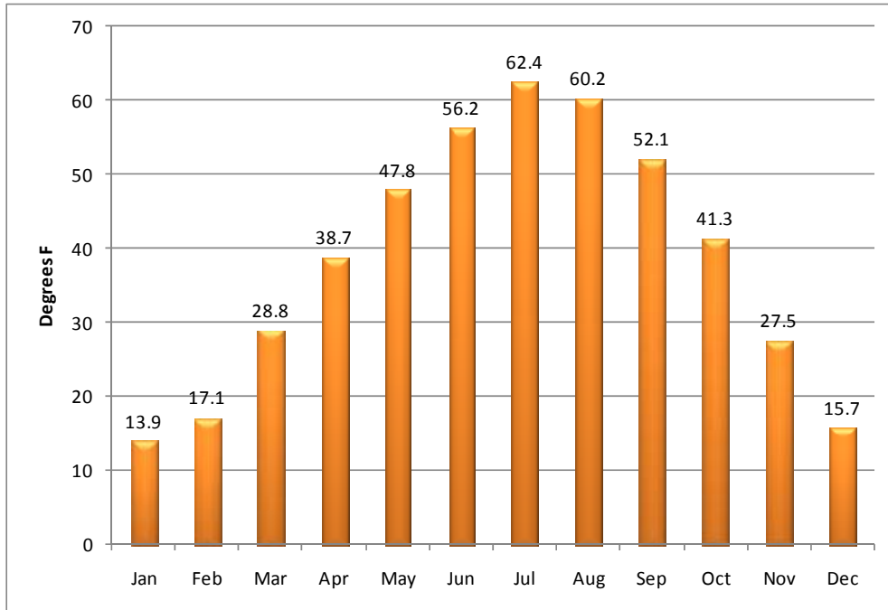
Figure 6 Average Mean Monthly Temperature Kremmling Climate Station 1950 through 2006
