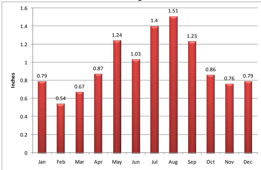
Figure 7 Average Mean Monthly Precipitation Kremmling Climate Station 1950 through 2006
