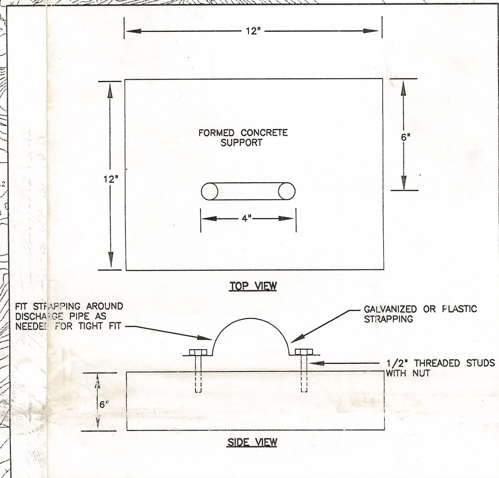
DETAIL 1A DISCHARGE LINE SUPPORT DETAIL
