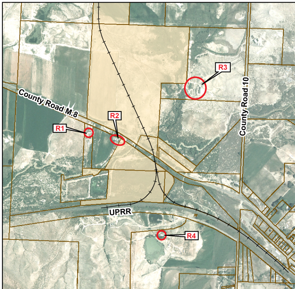
Figure 3-4 County Road M.8 / Railroad Grade Crossing Noise Sensitive Areas
