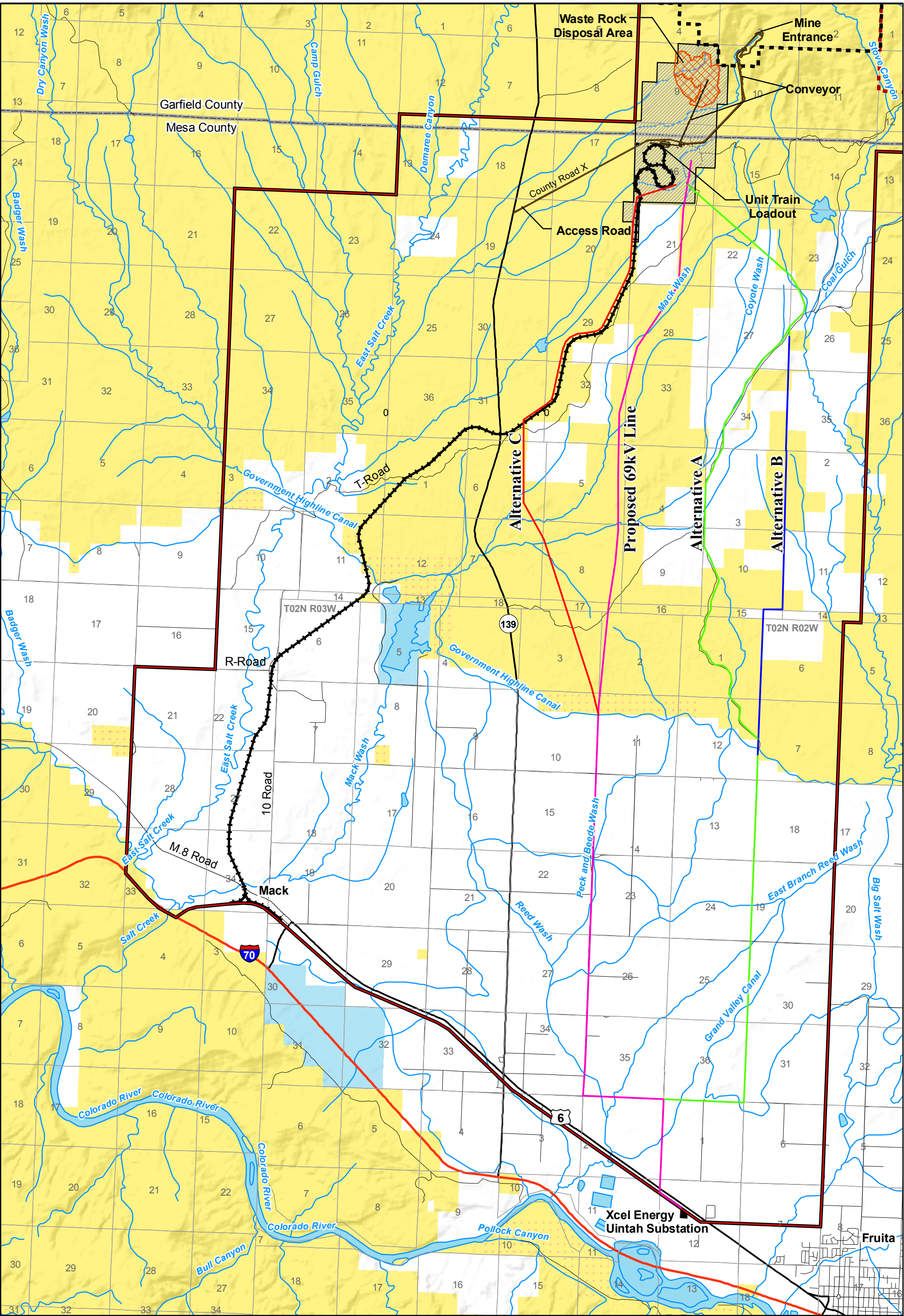
Figure 2-12 Transmission Line Alternatives
