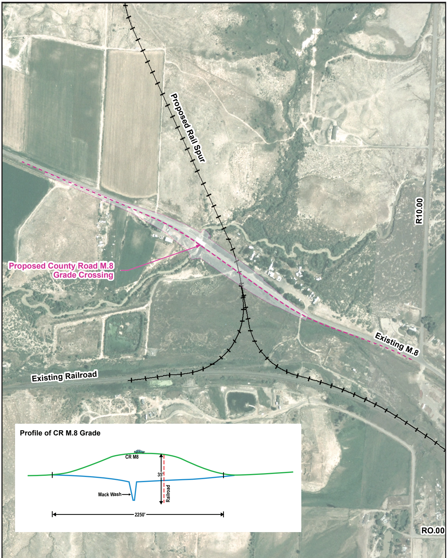
Figure 2-4 County Road M.8 Realignment
