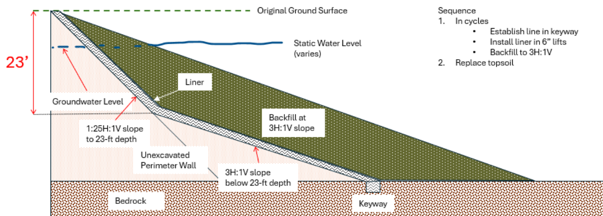
Figure 1. Typical Completed Reclamation Liner and Regraded Slope for Extraction Limit Wall 8
