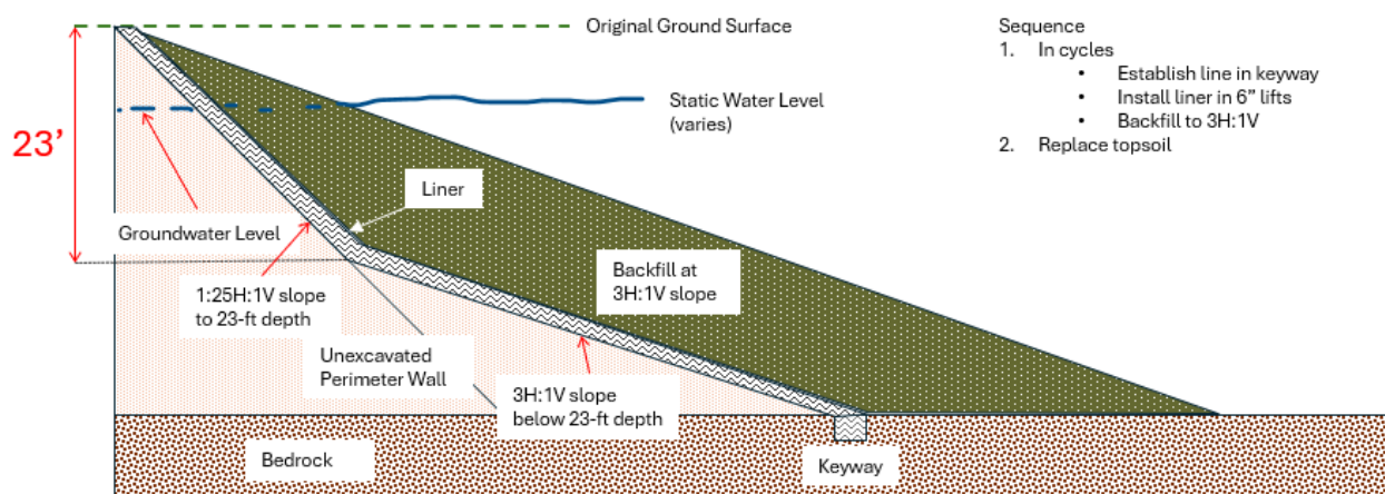
Figure 1. Typical Fully Reclaimed Liner and Backfill Construction
