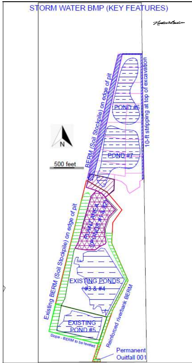
Figure D.3. Surface water management plan map
