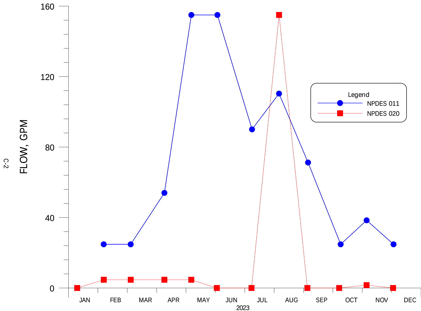
FIGURE C-2. FLOW VERSUS TIME FOR NPDES SITES 011 AND 020.
