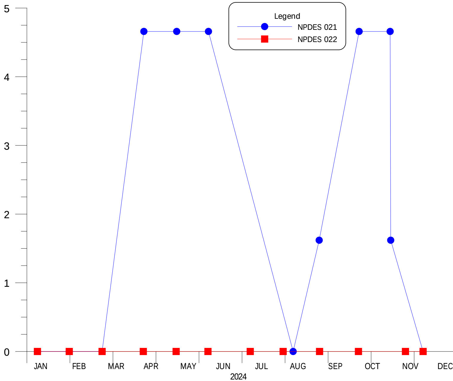
FIGURE C-3. FLOW VERSUS TIME FOR NPDES SITES 021 AND 022.
