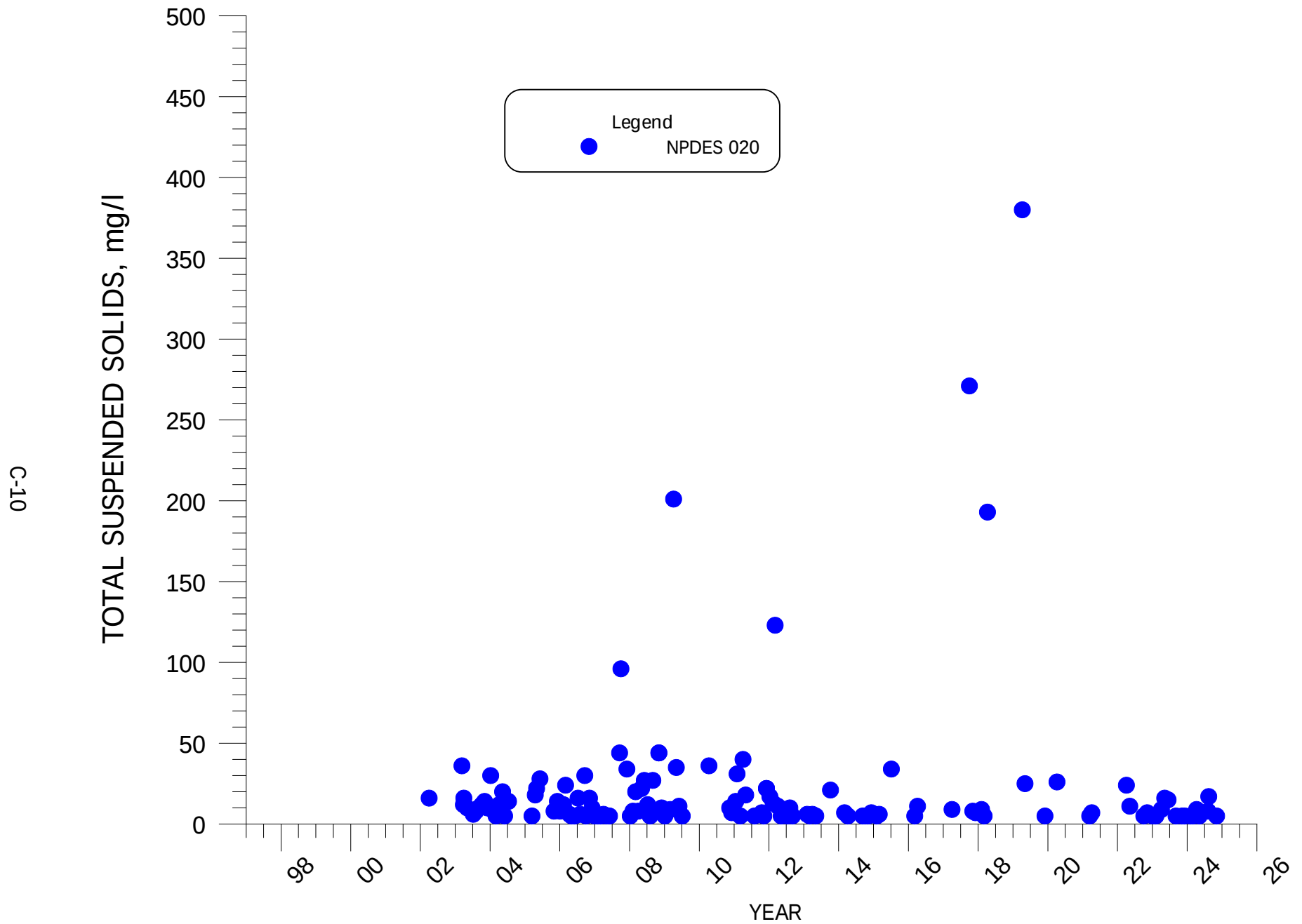
FIGURE C-10. TSS VERSUS TIME FOR NPDES SITE 020.
