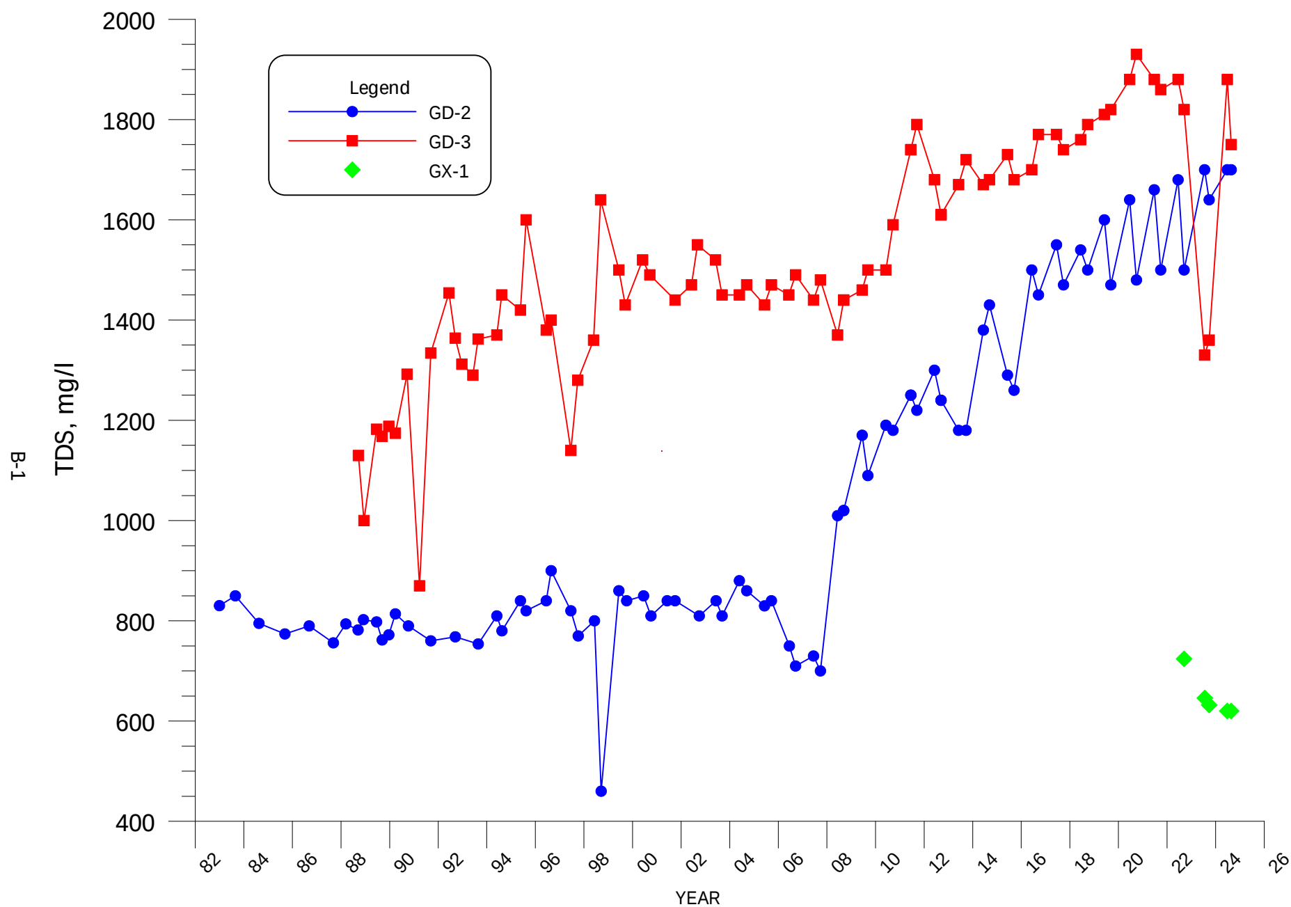
FIGURE B-1. TDS VERSUS TIME FOR WELLS GD-2, GD-3 AND GX-1.
