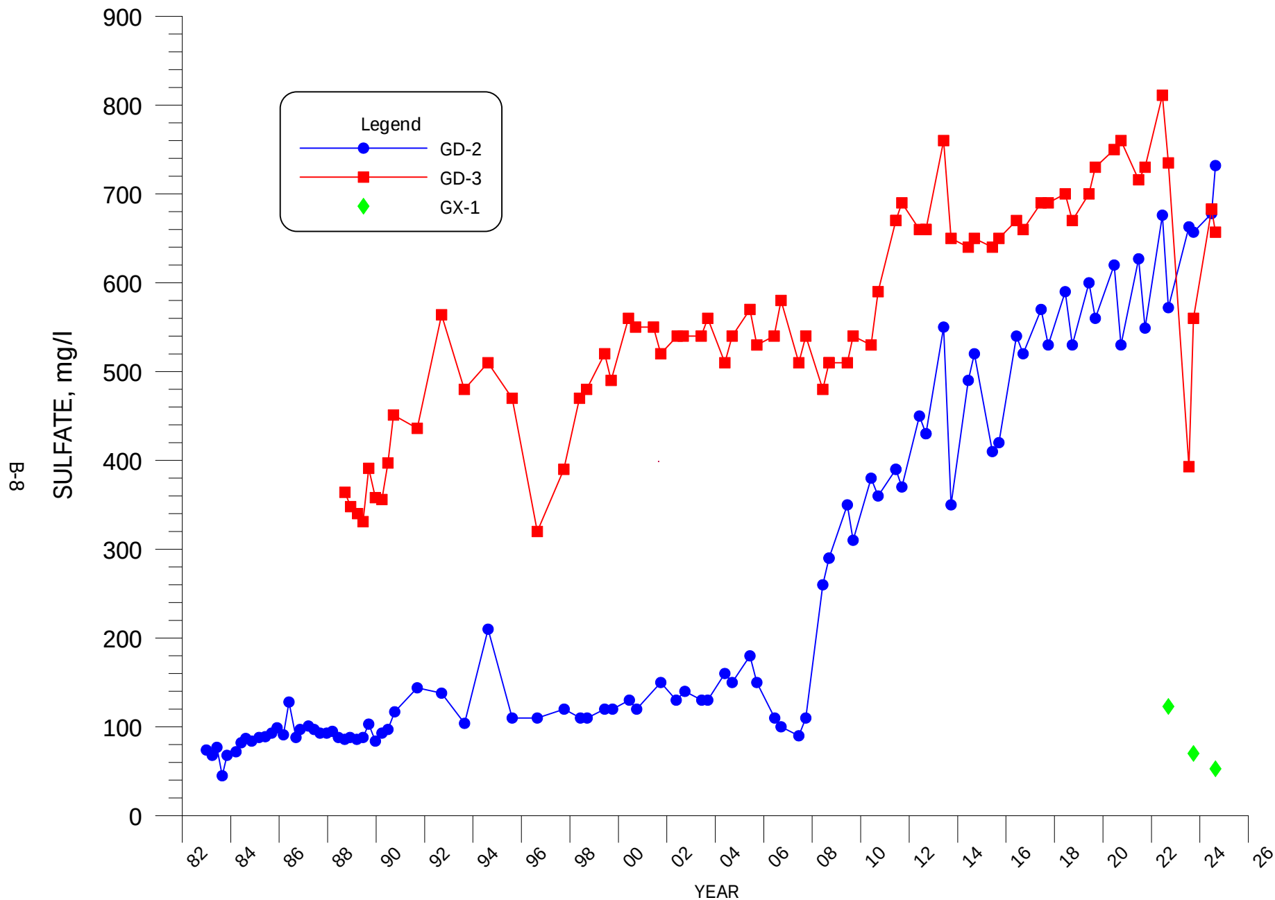
FIGURE B-8. SULFATE VERSUS TIME FOR WELLS GD-2, GD-3 AND GX-1.
