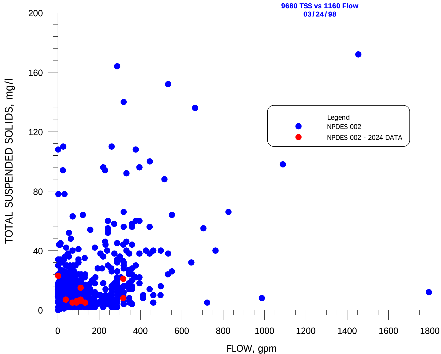
FIGURE C-7. FLOW VERSUS TSS FOR NPDES SITE 002.
