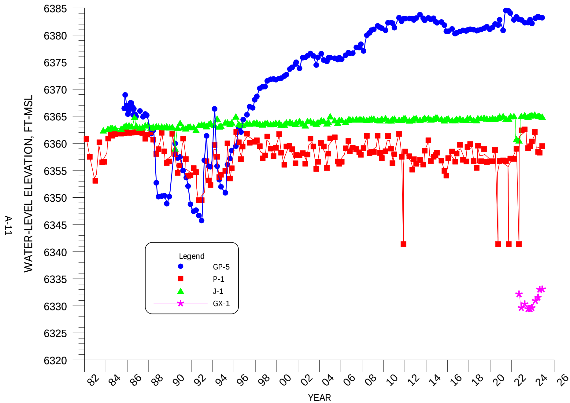
FIGURE A-11. WATER-LEVEL ELEVATION VERSUS TIME FOR WELLS GP-5, GX-1, P-1 AND J-1.
