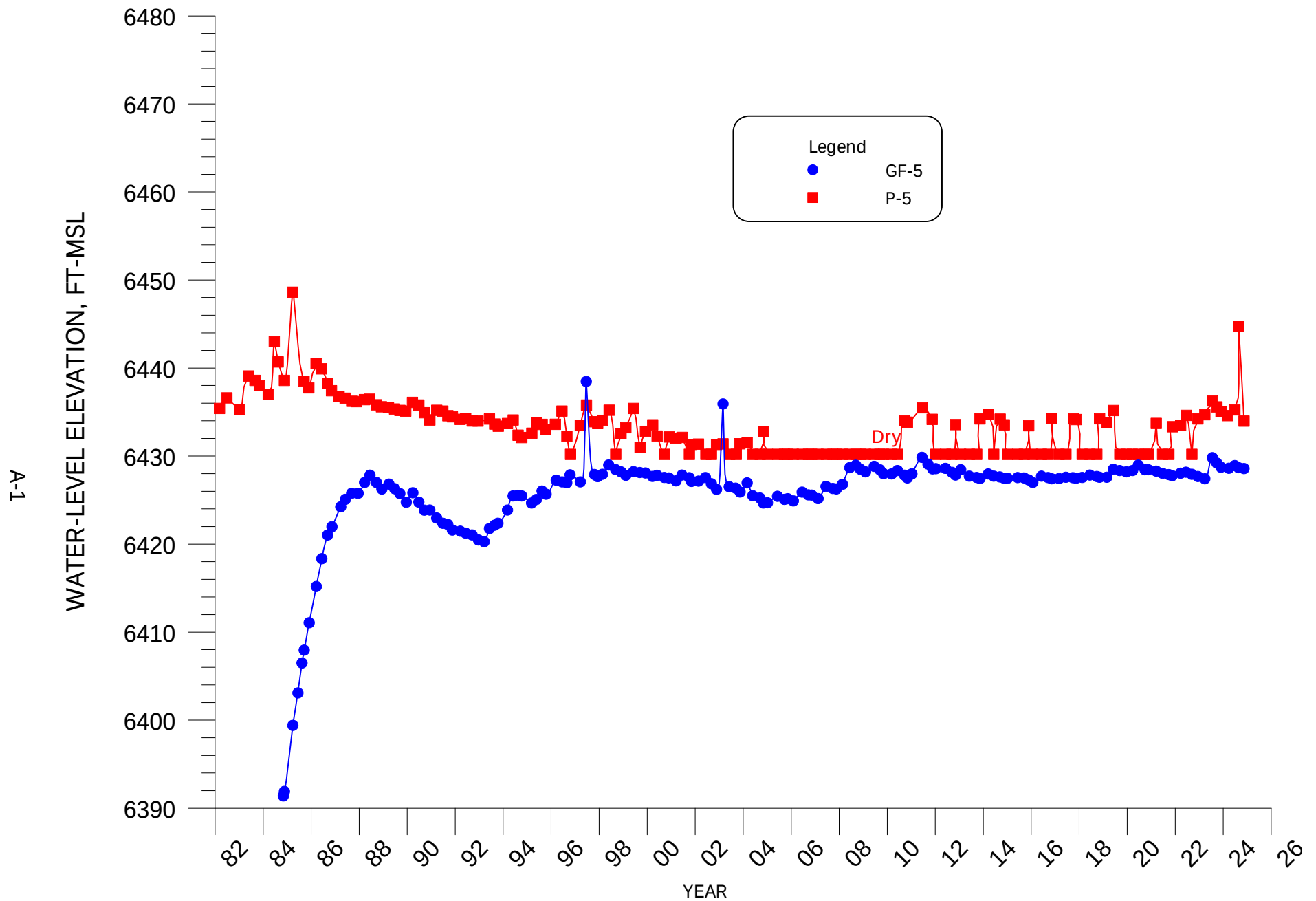
FIGURE A-1. WATER-LEVEL ELEVATION VERSUS TIME FOR WELLS GF-5 AND P-5.
