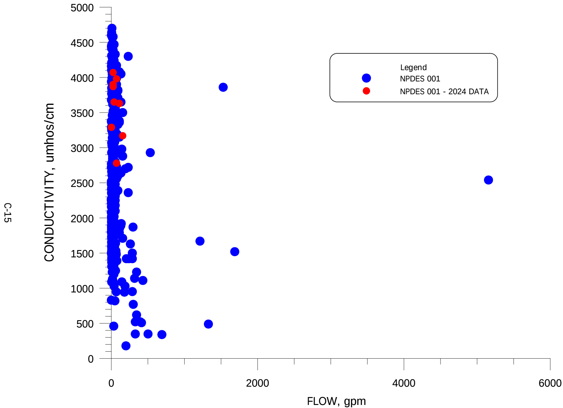
FIGURE C-15. FLOW VERSUS LAB CONDUCTIVITY FOR NPDES SITE 001.
