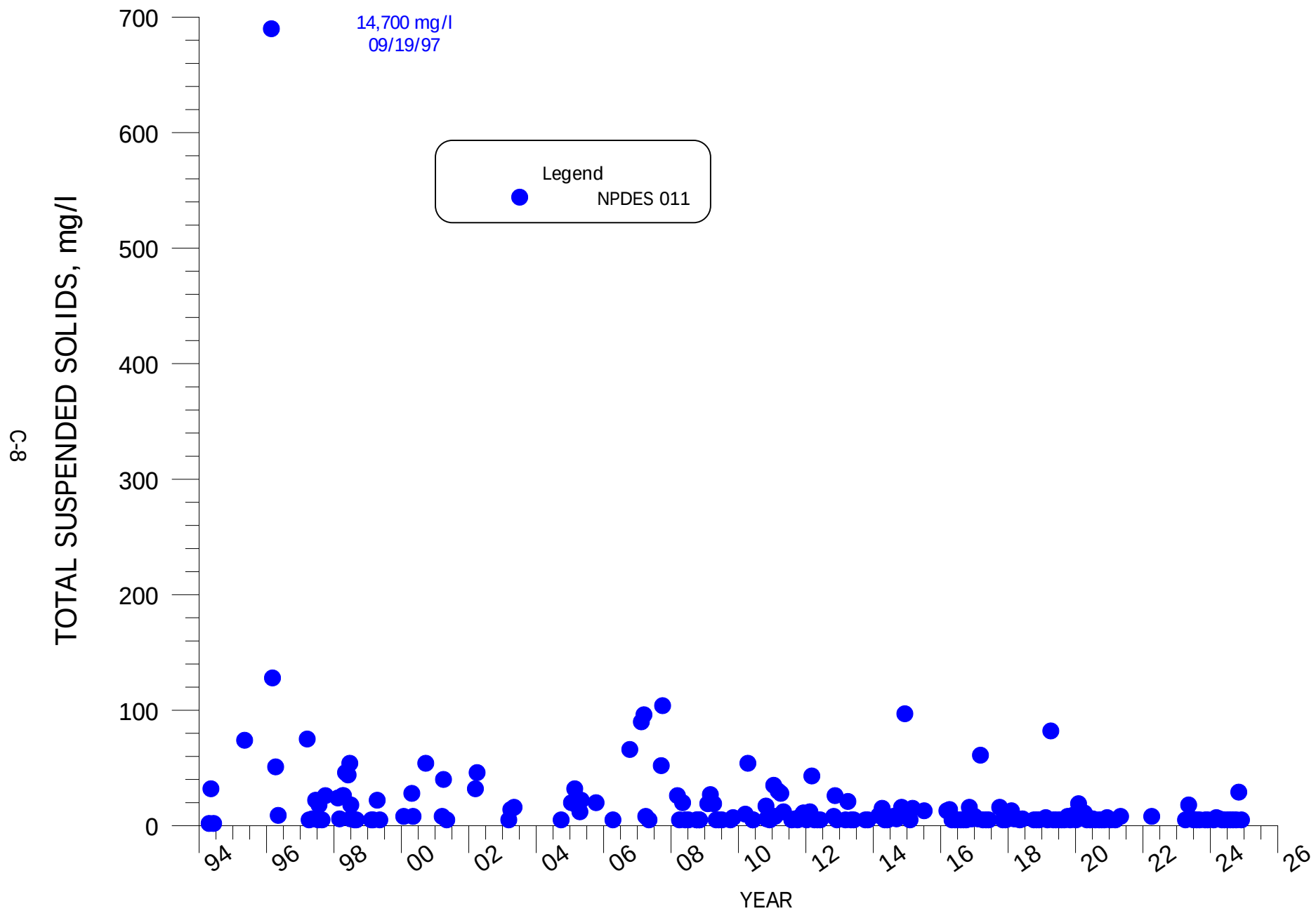
FIGURE C-8. TSS VERSUS TIME FOR NPDES SITE 011.
