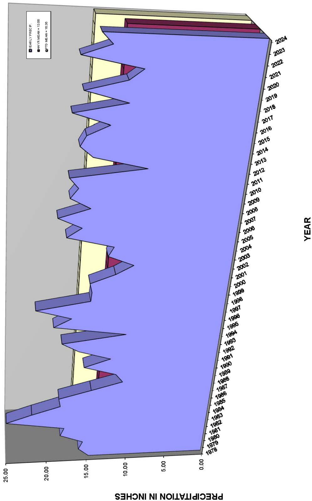
FIGURE 2-1. PRECIPITATION AT TRAPPER MINE 1978-2024
