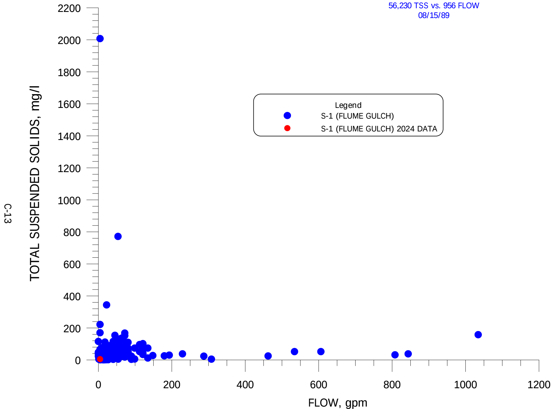
FIGURE C-13. FLOW VERSUS TSS FOR SITE S-1 (FLUME GULCH).
