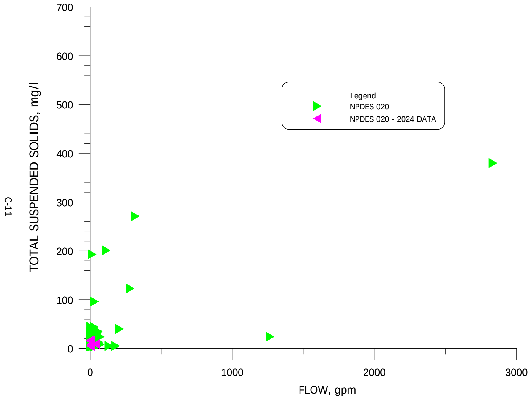
FIGURE C-11. FLOW VERSUS TSS FOR NPDES SITE 020.
