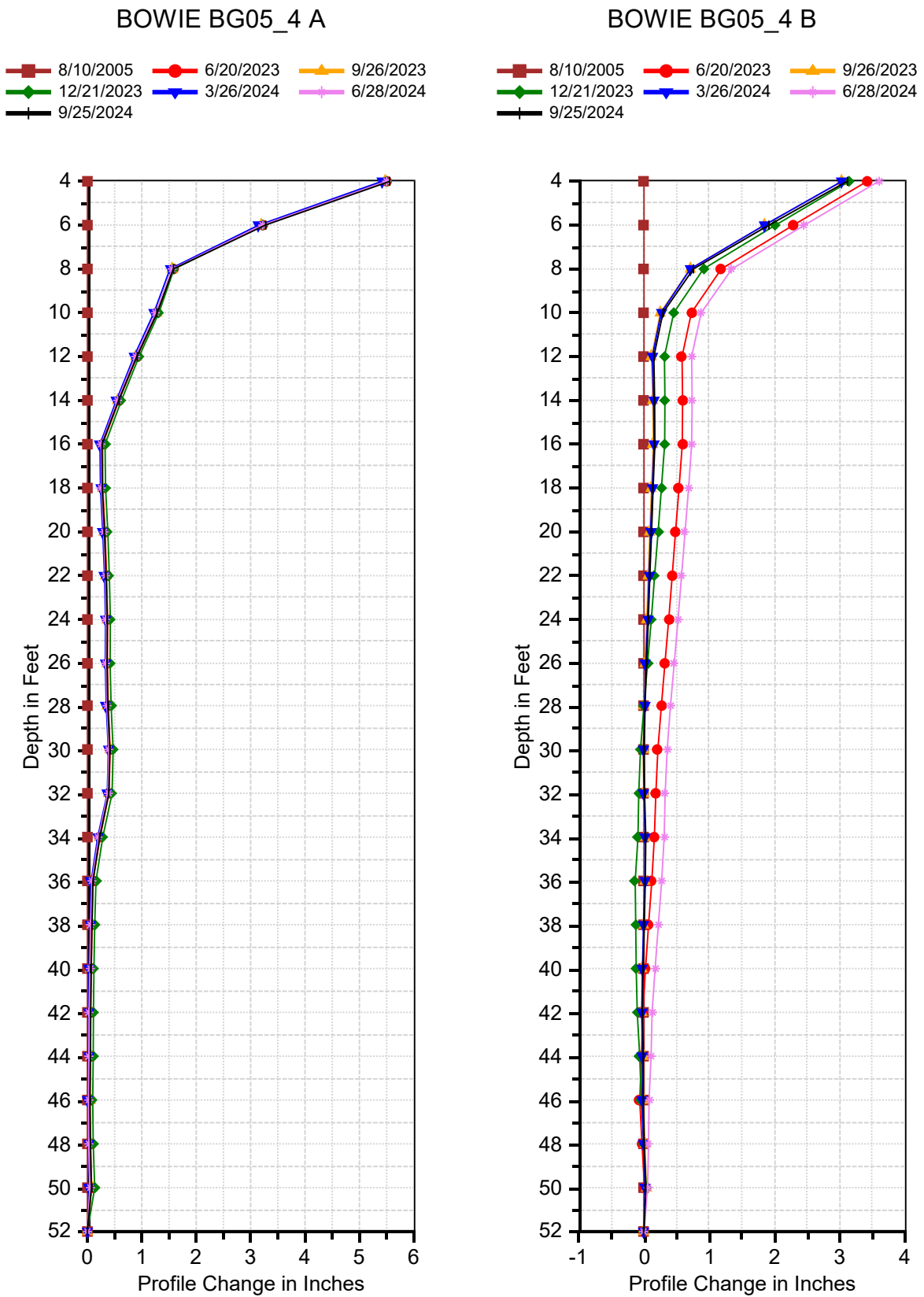
Figure 3 - Inclinomometer Displacement Curves
