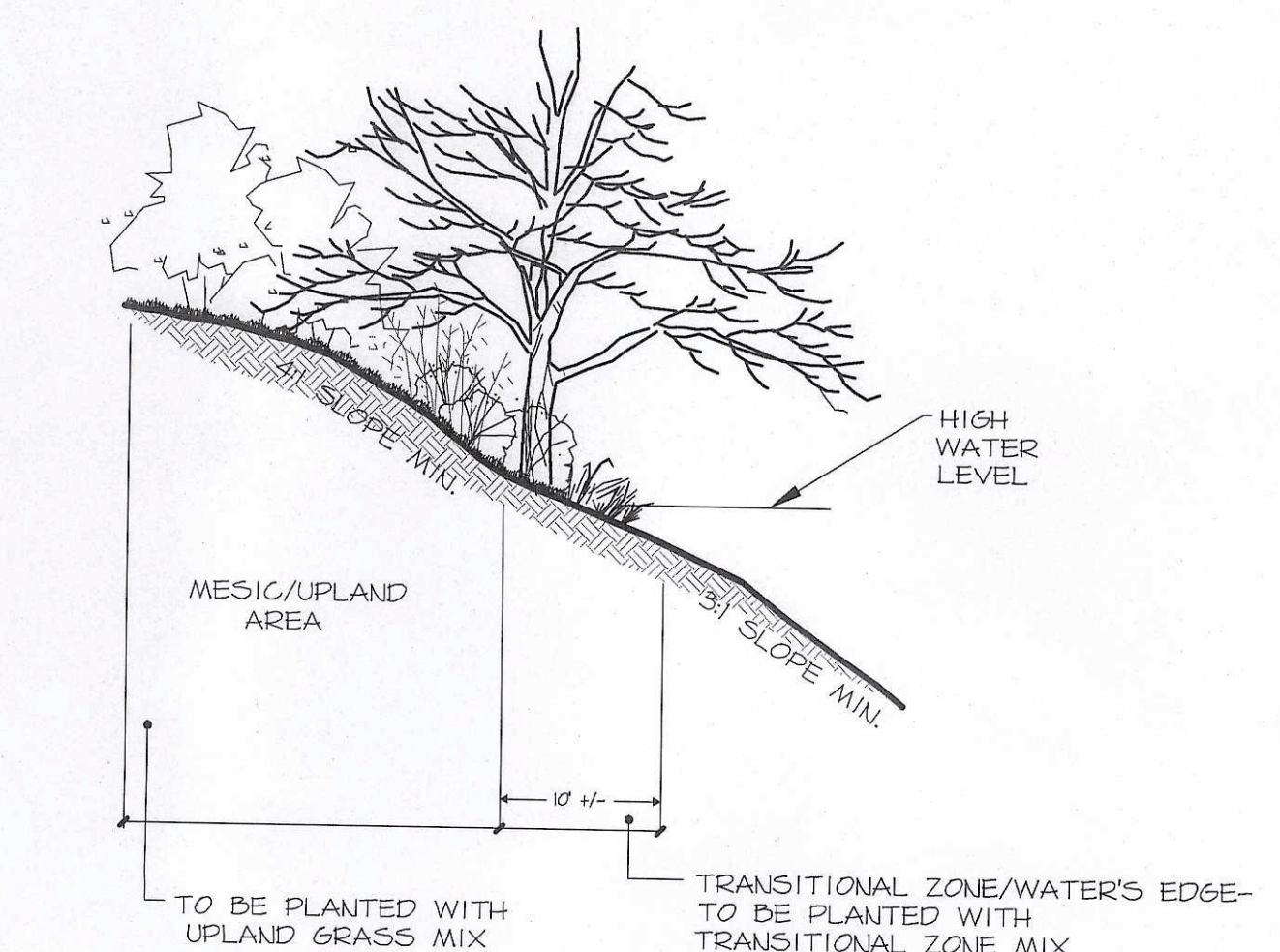
CROSS SECTION TYPICAL SHORELINE PLANTING DETAIL NOT TO SCALE
