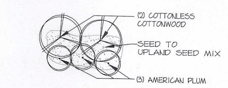
TYPICAL BERM PLANTING DETAIL NOT TO SCALE
