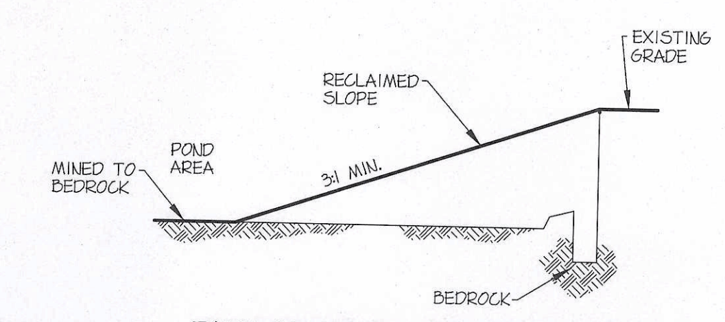
RECLAMATION CROSS SECTION NOT TO SCALE
