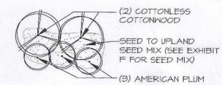
TYPICAL BERM PLANTING DETAIL
