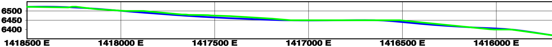
CROSS - SECTION I EAST PIT N 412000
