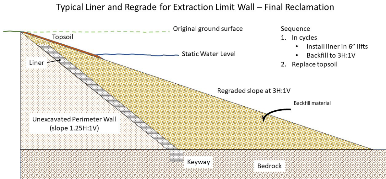
Typical Liner and Regrade for Extraction Limit Wall
