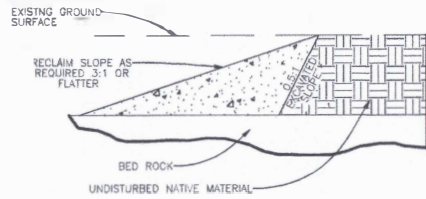
TYPICAL CROSS SECTION (PRIOR TO BACKFILL)
