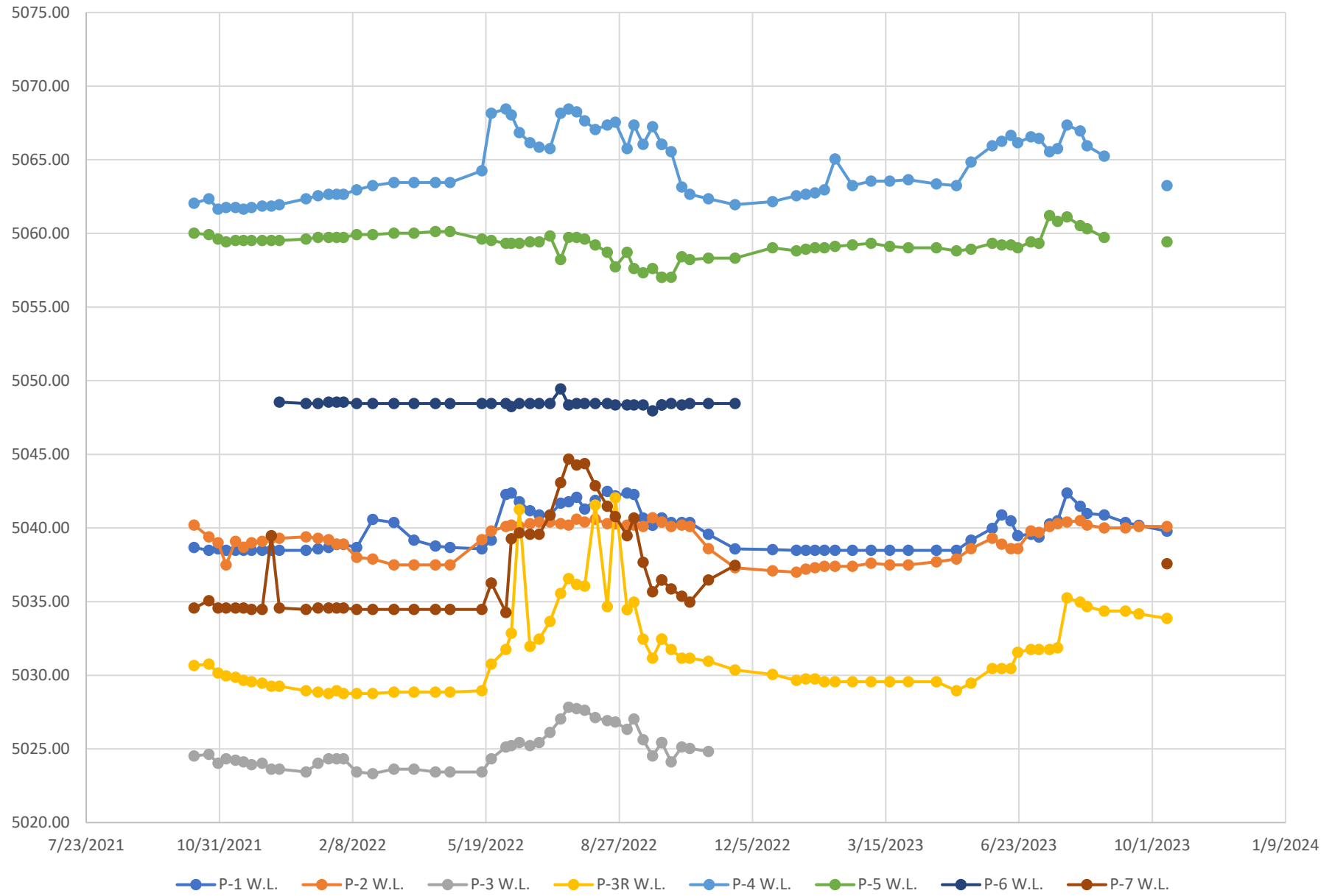
GOOSE HAVEN GROUNDWATER LEVELS 10-12-2021 THRU 10-12-2023
