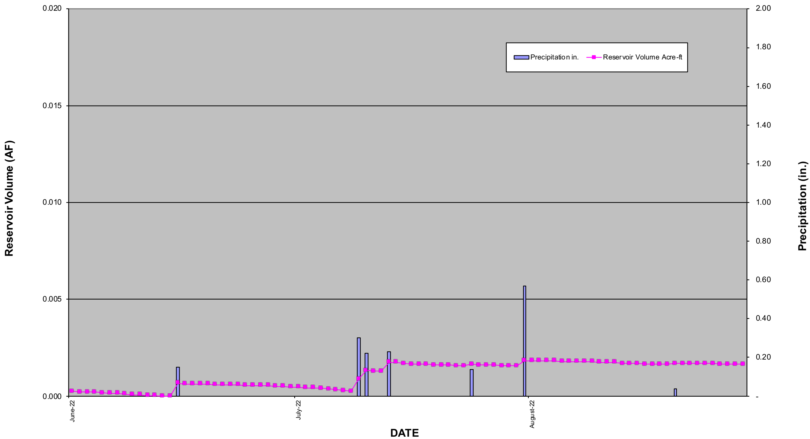
Reservoir Volume and Precipitation During 90-Day Initial Liner Test
