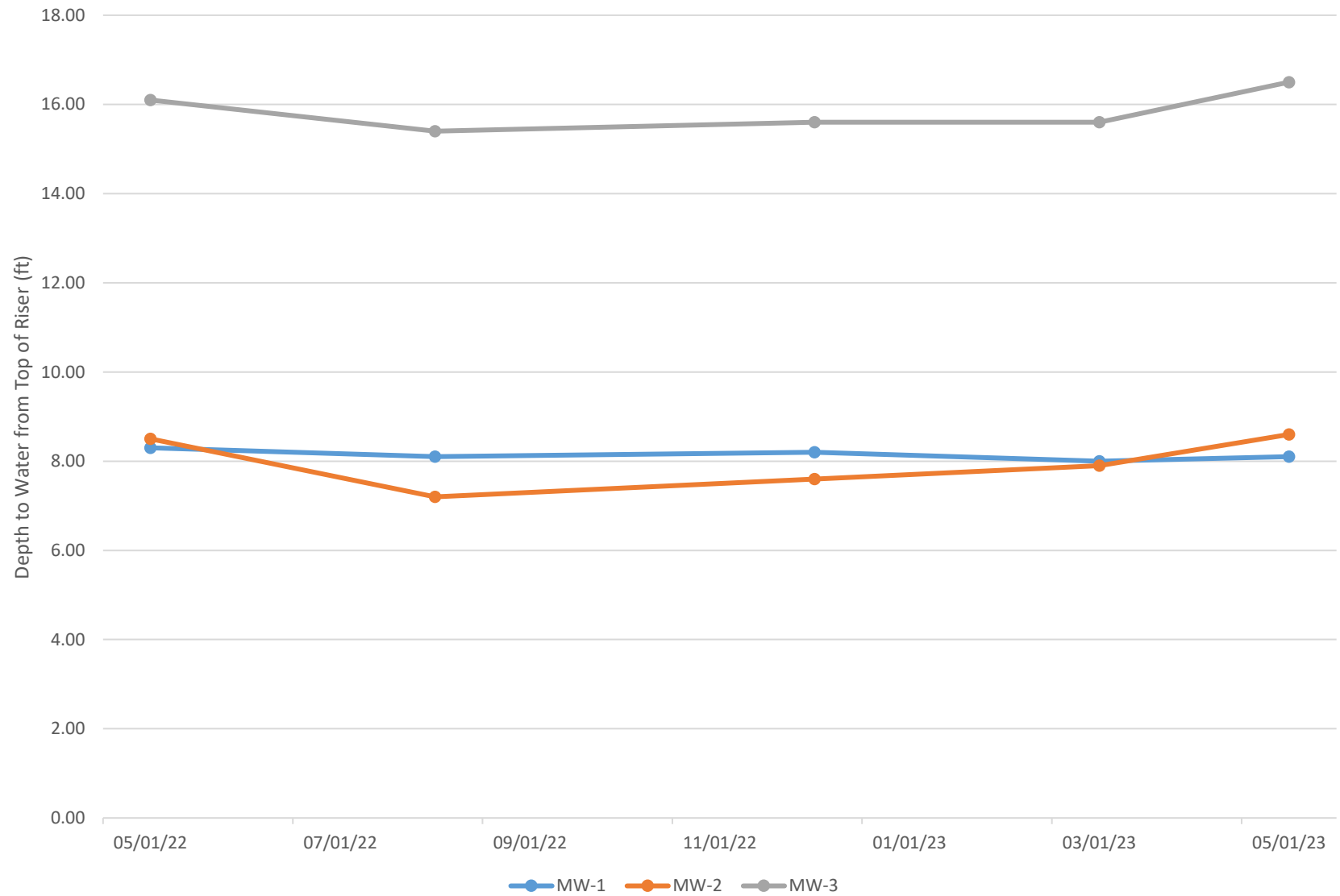
Platte Valley Monitoring Well Data 05/31/22 - 05/04/23
