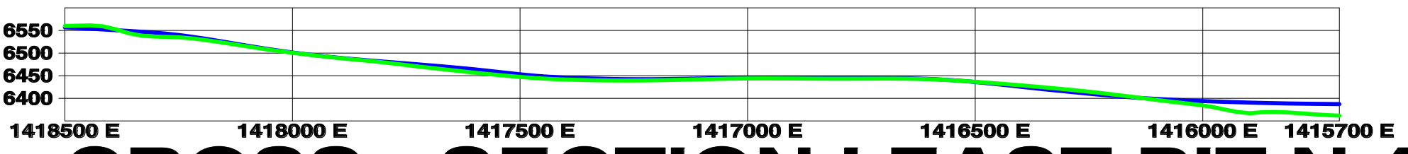
CROSS - SECTION I EAST PIT N 411100
