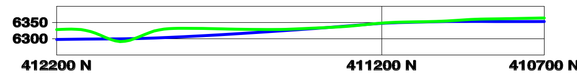
CROSS - SECTION I WEST PIT E 1409900
