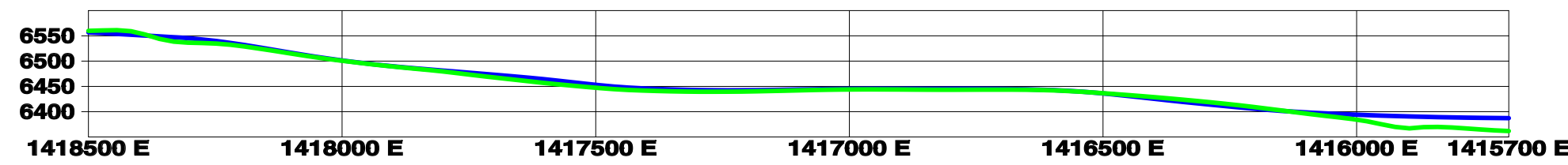
CROSS - SECTION I EAST PIT N 411100
