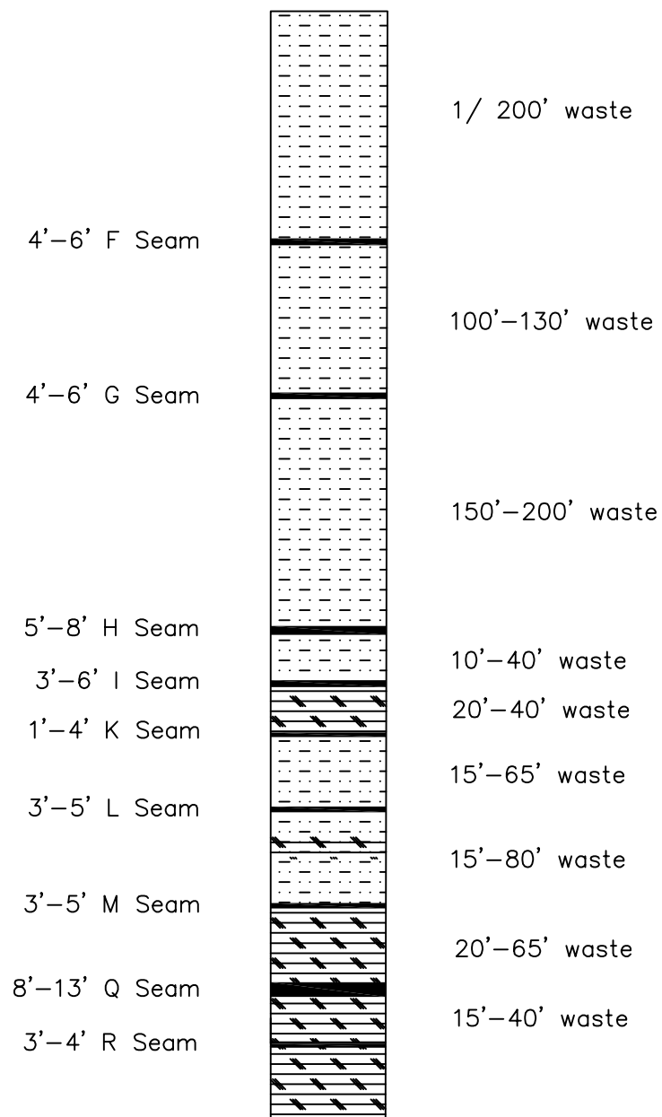
FIGURE 2.7-5 TYPICAL STRATIGRAPHIC SECTION OF THE TRAPPER MINE AREA NOT TO SCALE 1/ waste is interburden and overburden
