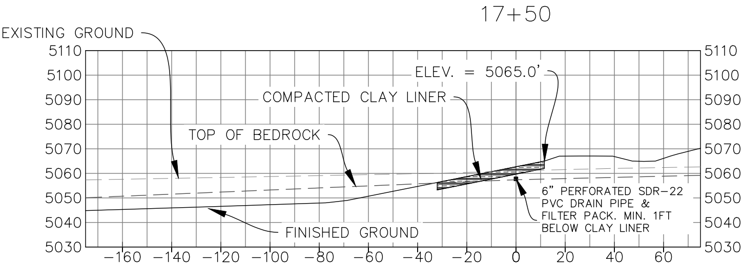
TYPICAL SOUTH UNDERDRAIN CROSS SECTION WHERE DRAIN OCCURS UNDER CLAY LINER
