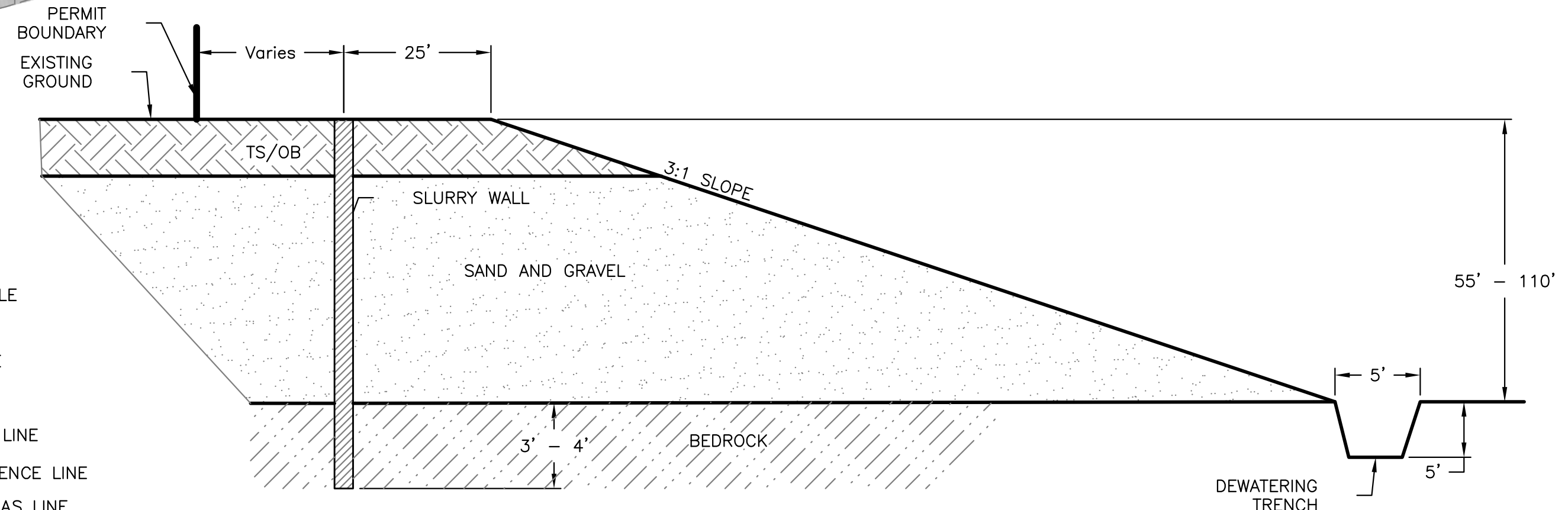
TYPICAL MINING SECTION N.T.S.
