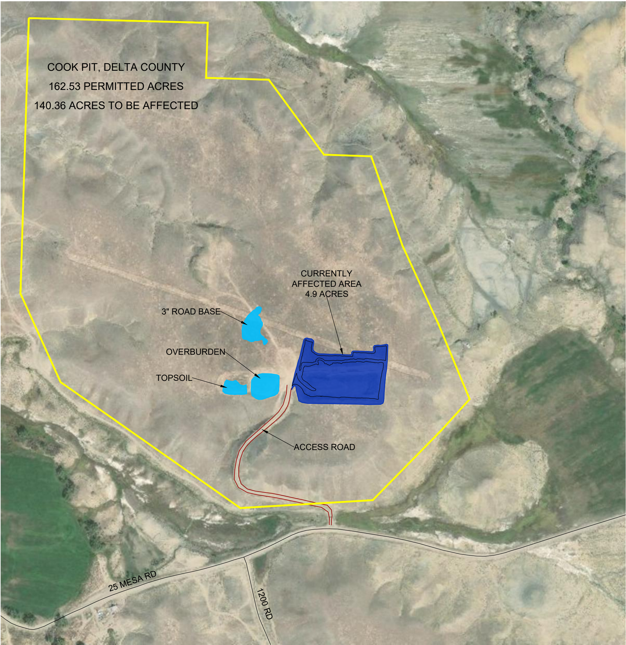
VICINITY MAP
