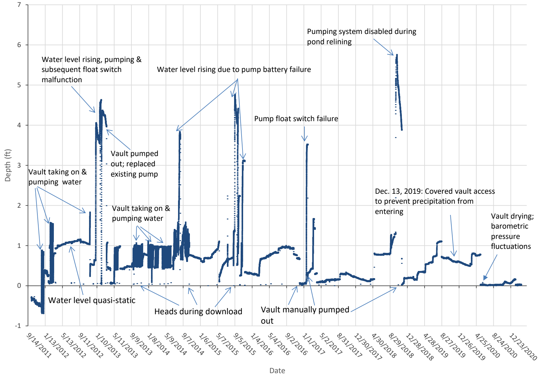
Figure 7. Logan Wash Mine Evaporation Pond Leak Detection Vault Water Levels
