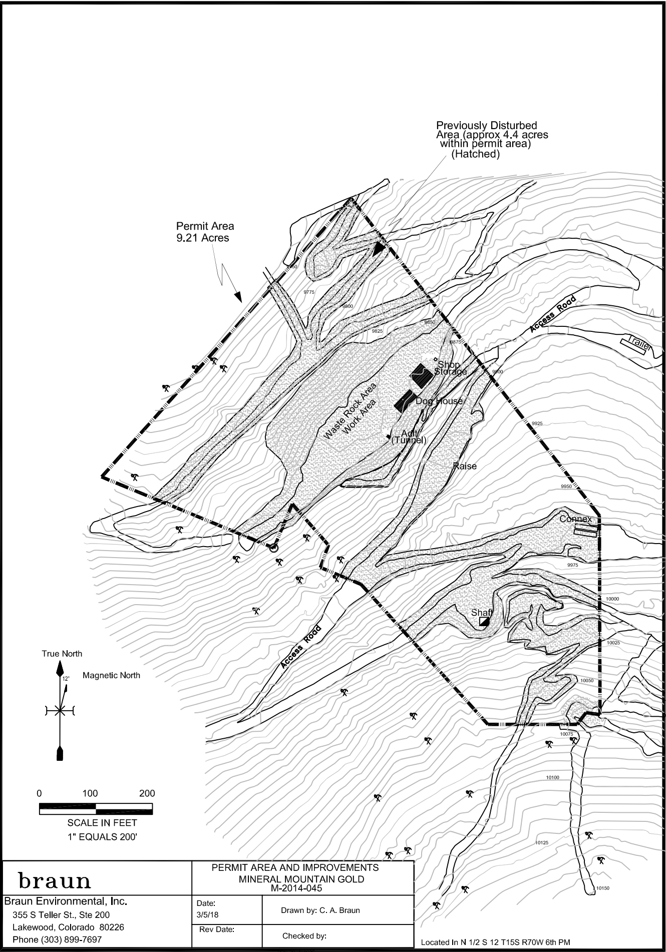
SITE MAP SHOWING PERMITTED AREA AND FEATURES
