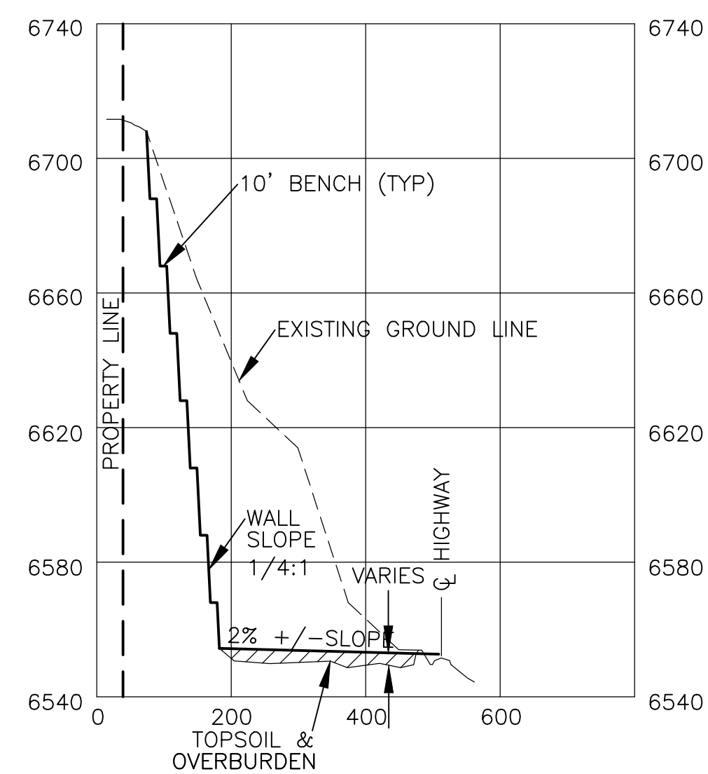
PHASE 2 HIGHWALL PROFILE HORIZ. 1"=200' VERT. 1"=40'
