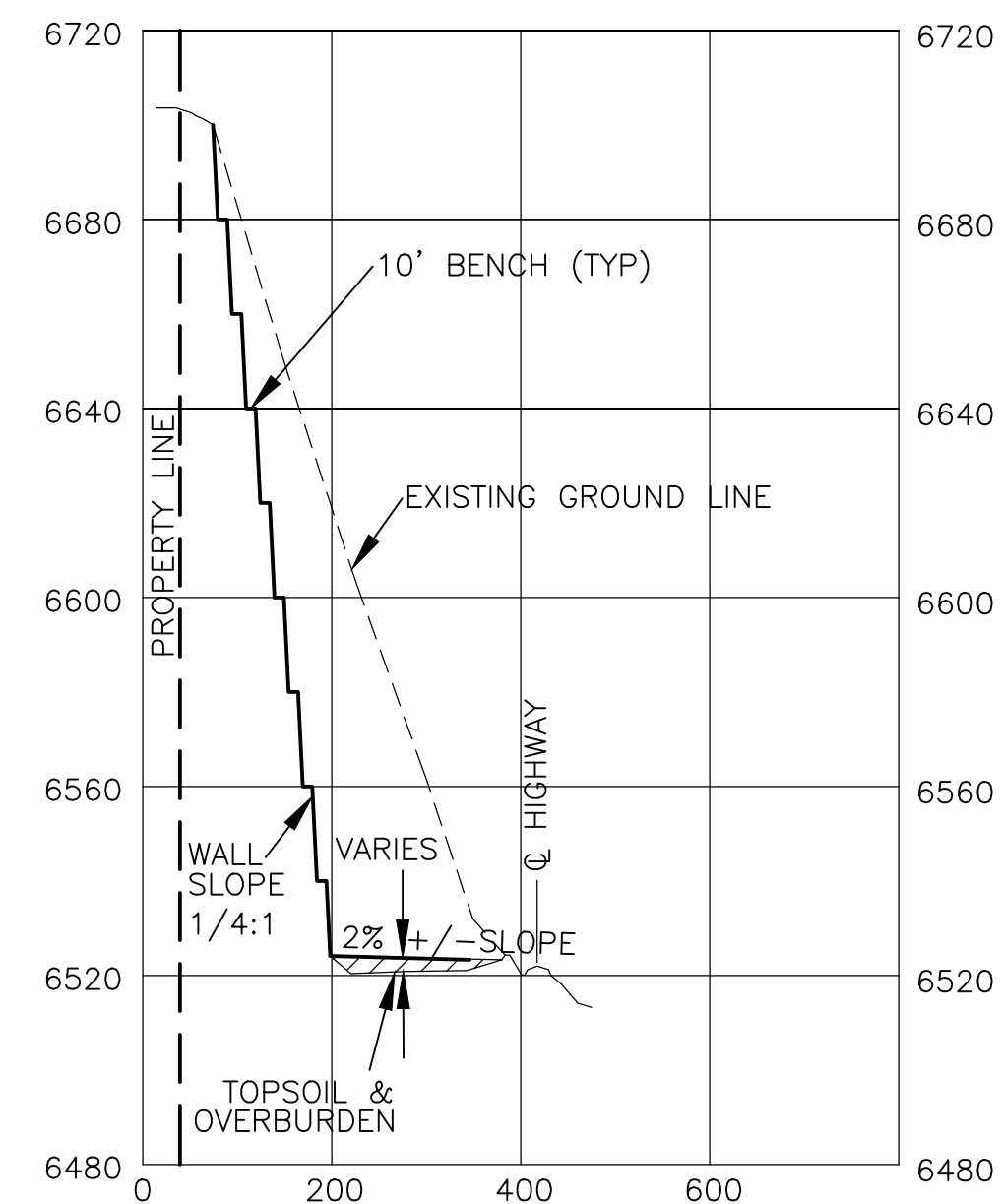
PHASE 3 HIGHWALL PROFILE HORIZ. 1"=200' VERT. 1"=40'
