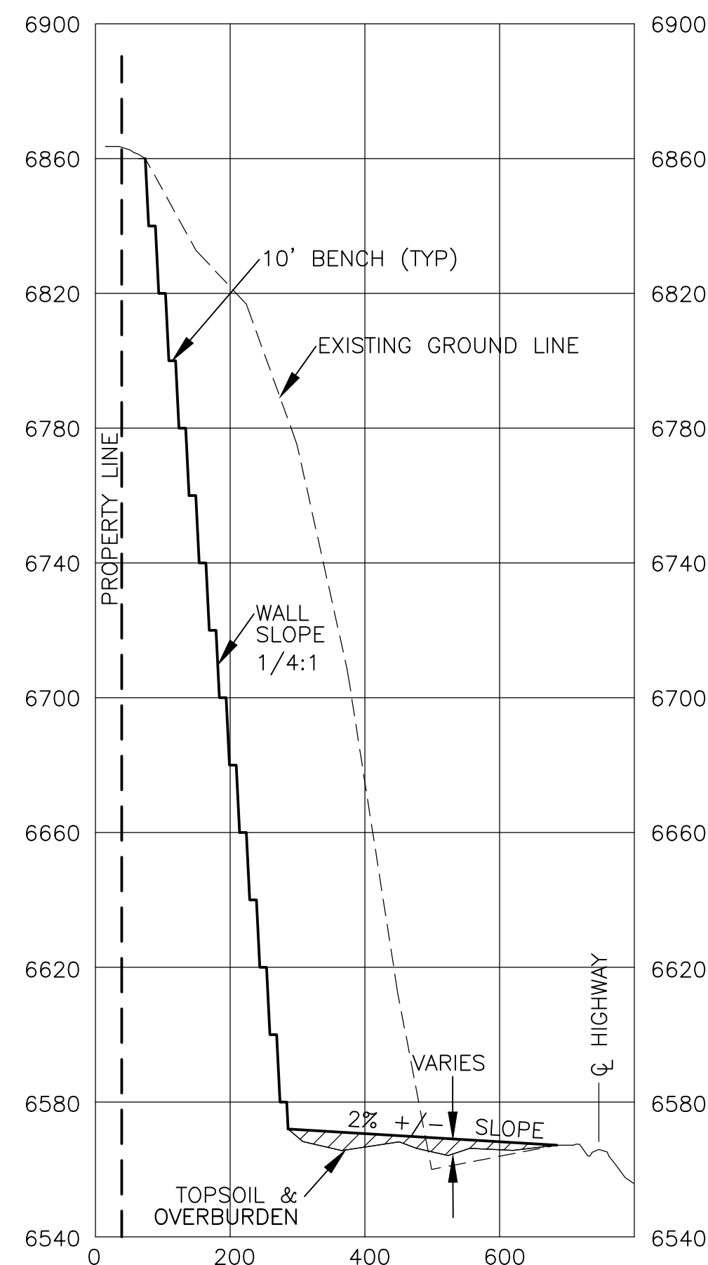
PHASE 1 HIGHWALL PROFILE HORIZ. 1"=200' VERT. 1"=40'
