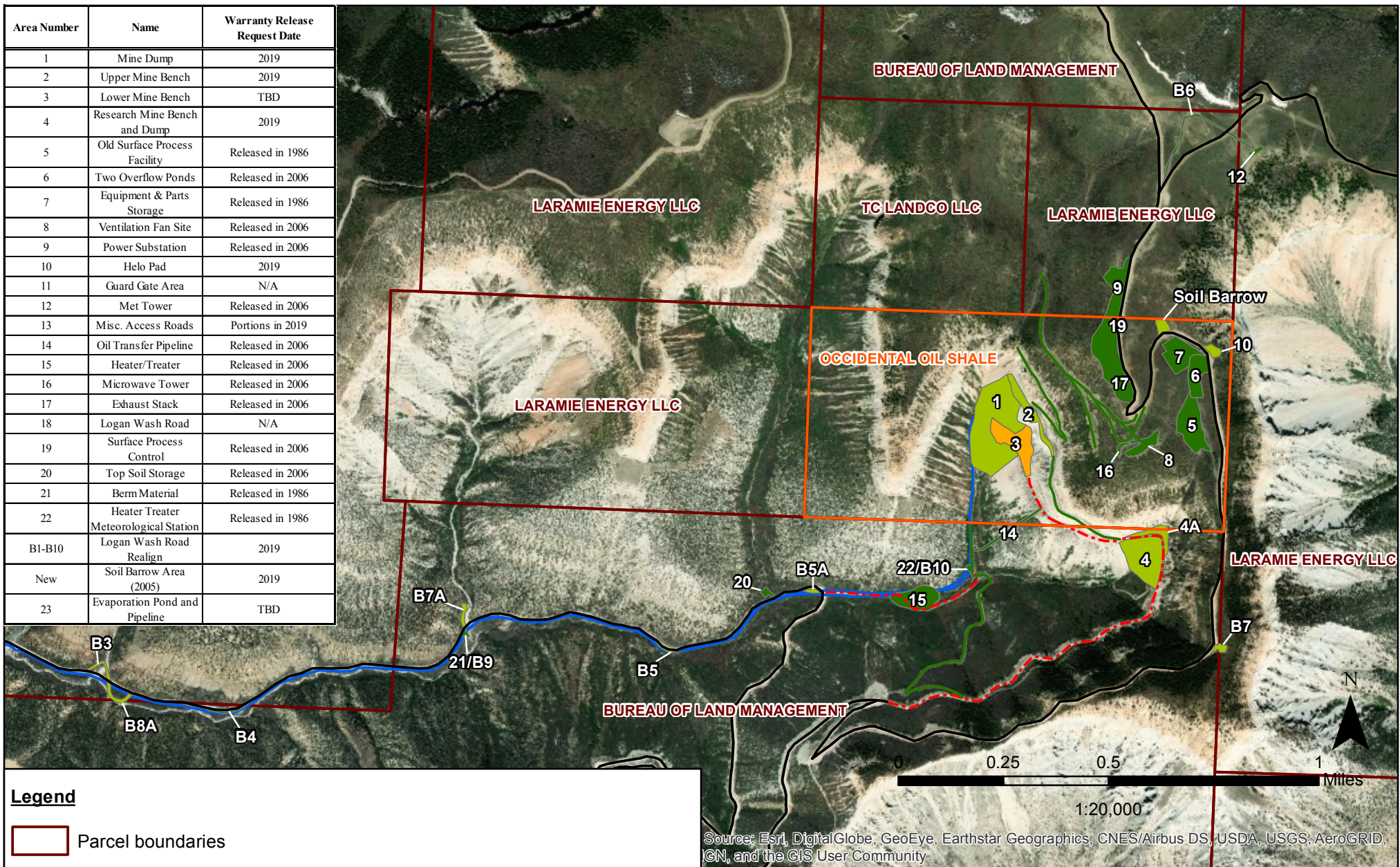
Figure 4A. Logan Wash Mine Reclamation Status
