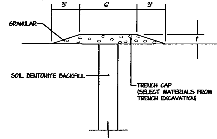
SLURRY WALL CAP DETAIL
