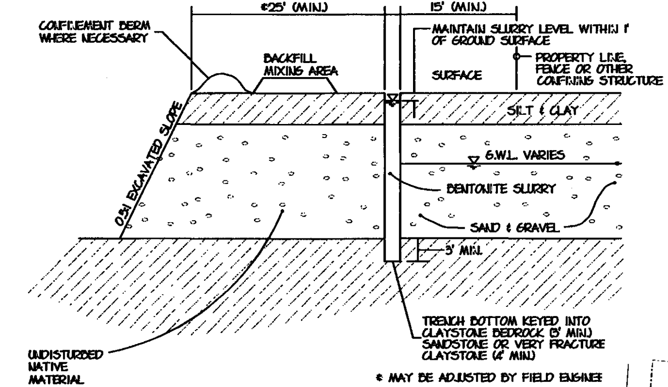
TYPICAL SLURRY WALL CROSS SECTION (PRIOR TO BACKFILL)
