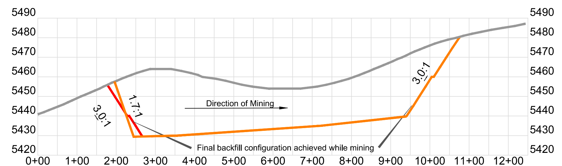
Section B-B'
