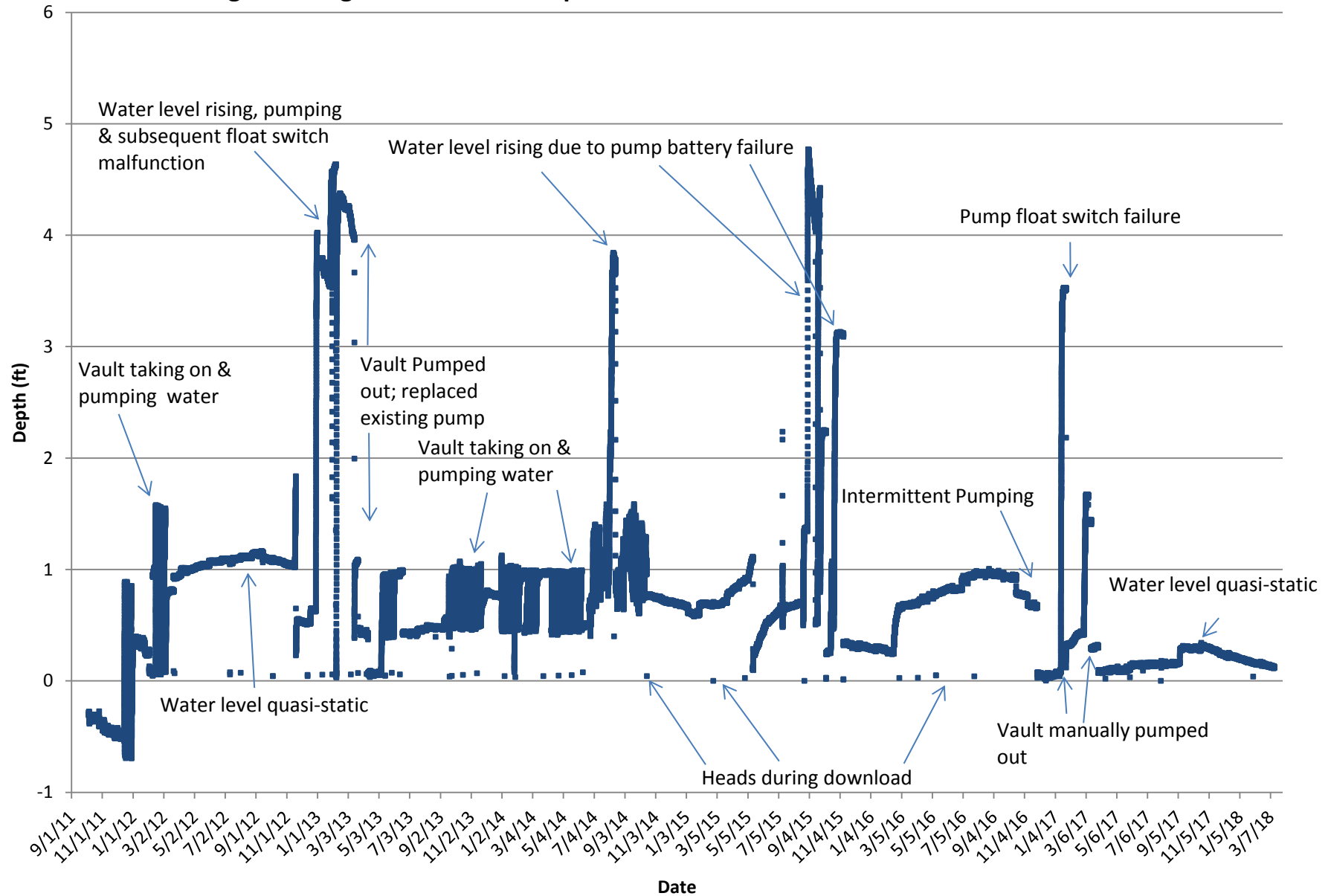
Figure 7. Logan Wash Mine Evaporation Pond Leak Detection Vault Water Levels
