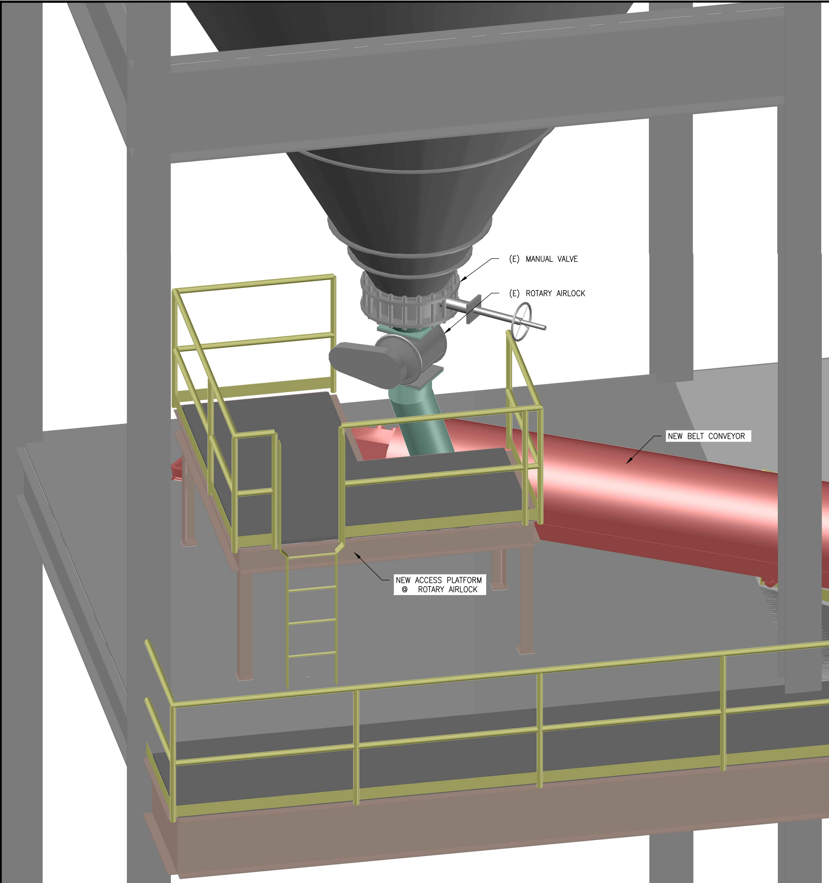
ISOMETRIC VIEW AT F&I DISCHARGE SCALE: NTS
