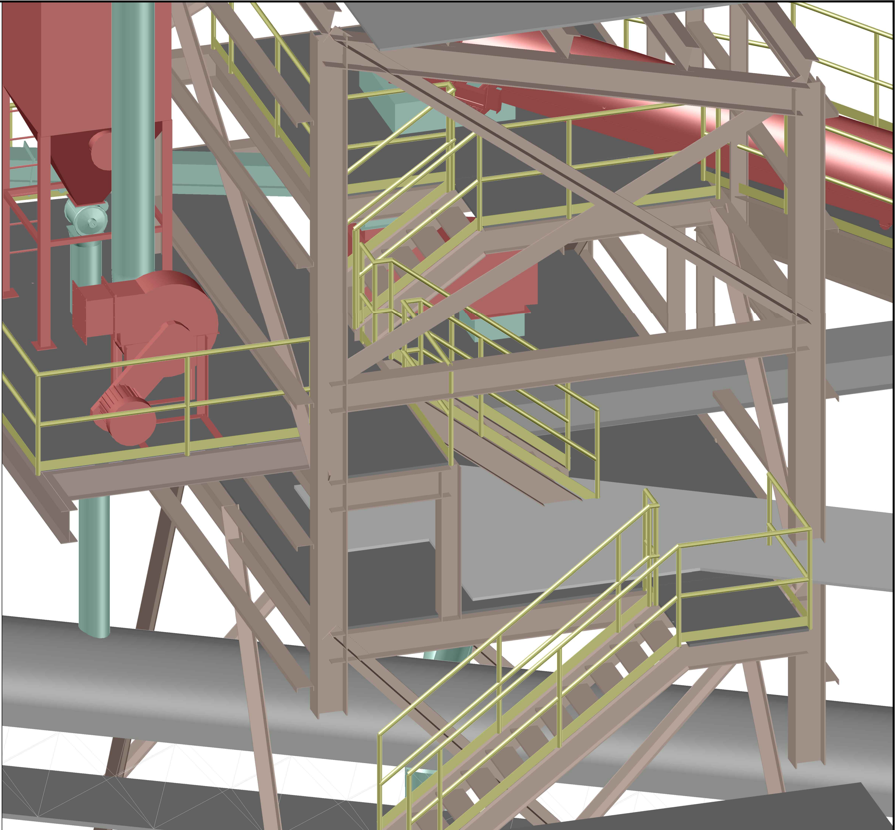
ISOMETRIC AT ACCESS STAIR SCALE: NTS
