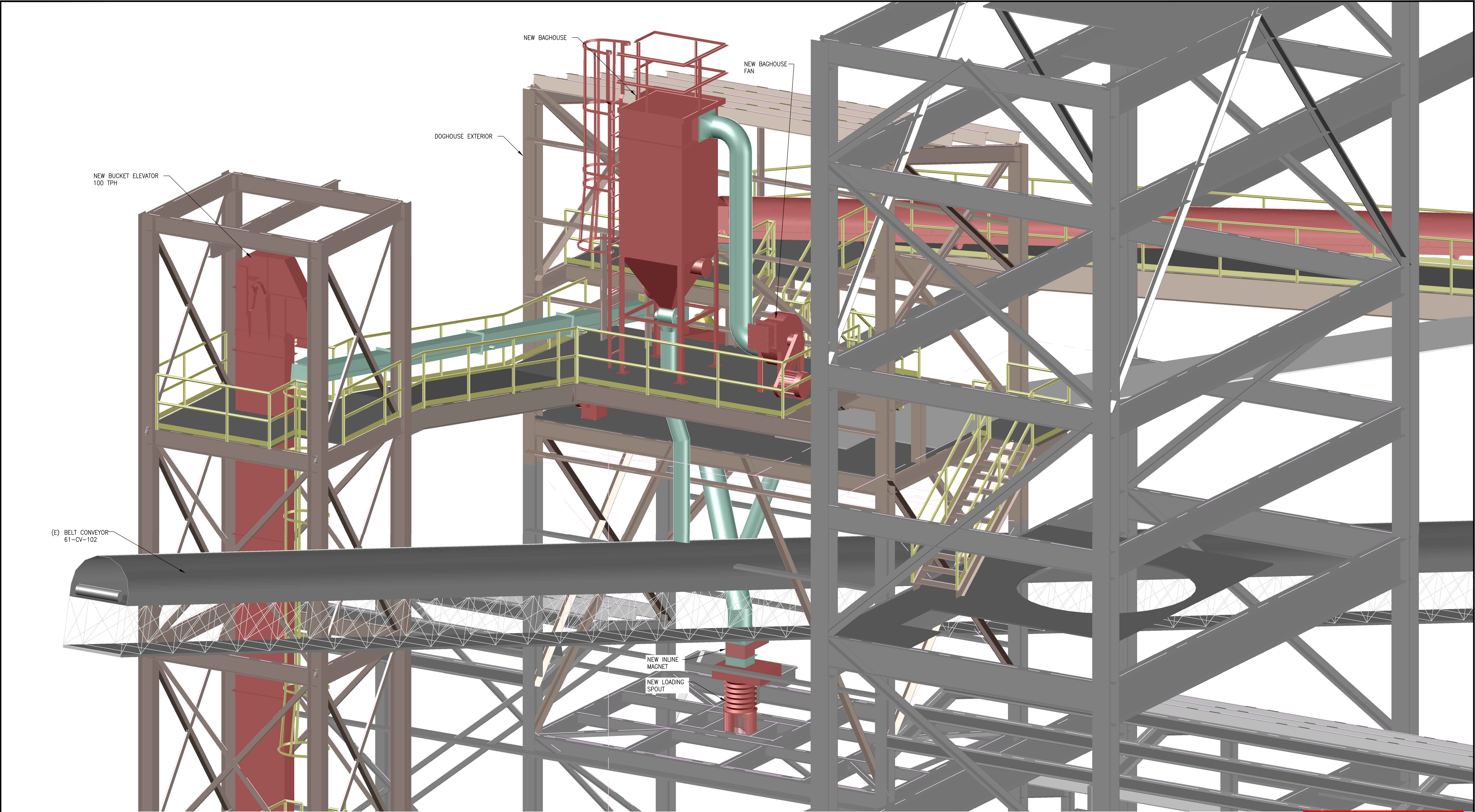
ISOMETRIC LOOKING NW SCALE: NTS
