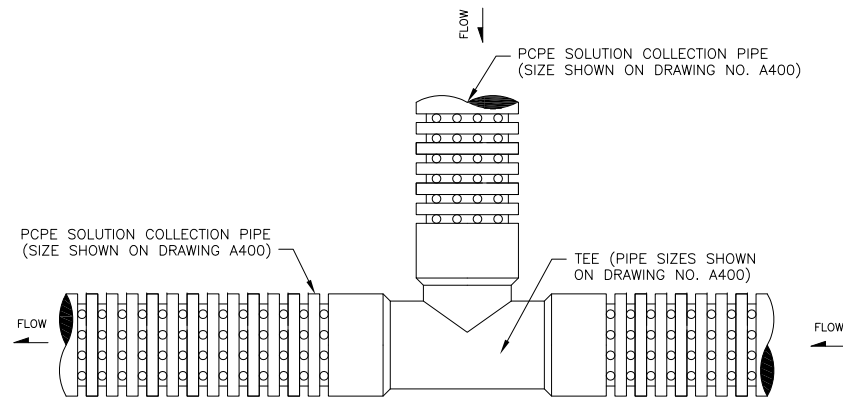
29 A400 ALTERNATIVE SOLUTION COLLECTION PIPE TEE JUNCTION NTS
