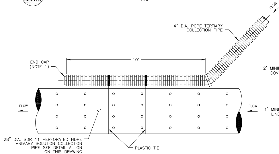
33 A400 TYPICAL TERTIARY OR SECONDARY TO PRIMARY SOLUTION COLLECTION PIPE CONNECTION NTS
