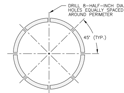
AL A410 PRIMARY SOLUTION COLLECTION PIPE PERFORATION DETAIL NTS
