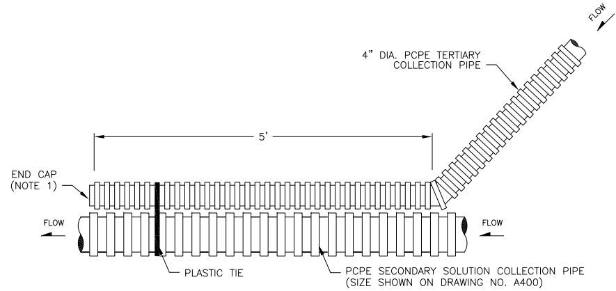
28 A400 TYPICAL SINGLE TERTIARY TO SECONDARY SOLUTION COLLECTION PIPE JUNCTION NTS
