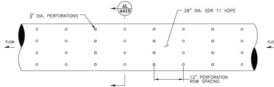
31 A400 PRIMARY SOLUTION COLLECTION PIPE NTS
