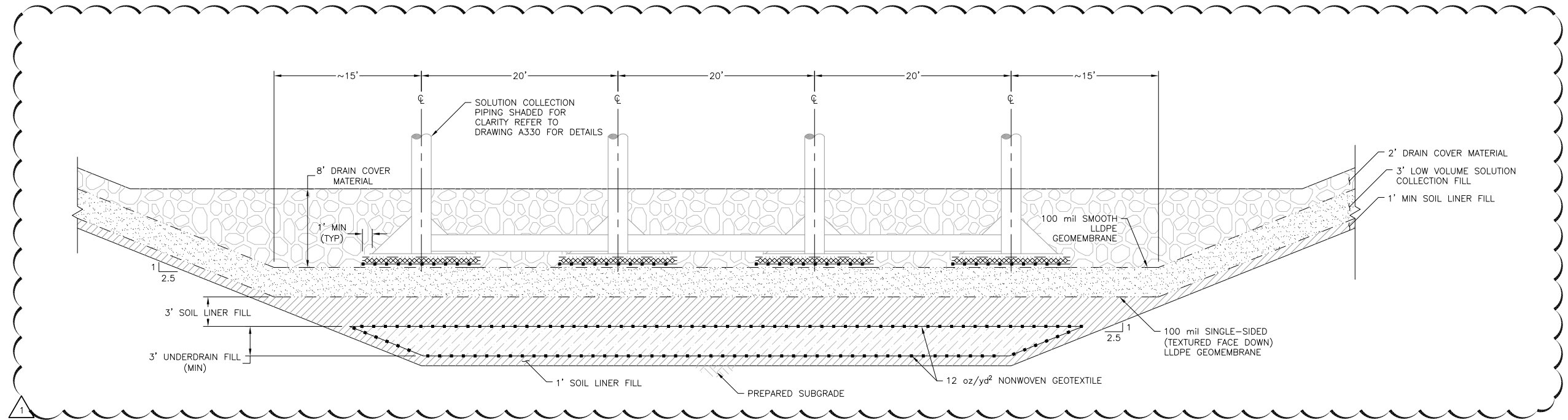
AG NORTHWEST-SOUTHEAST SECTION A330 NTS
