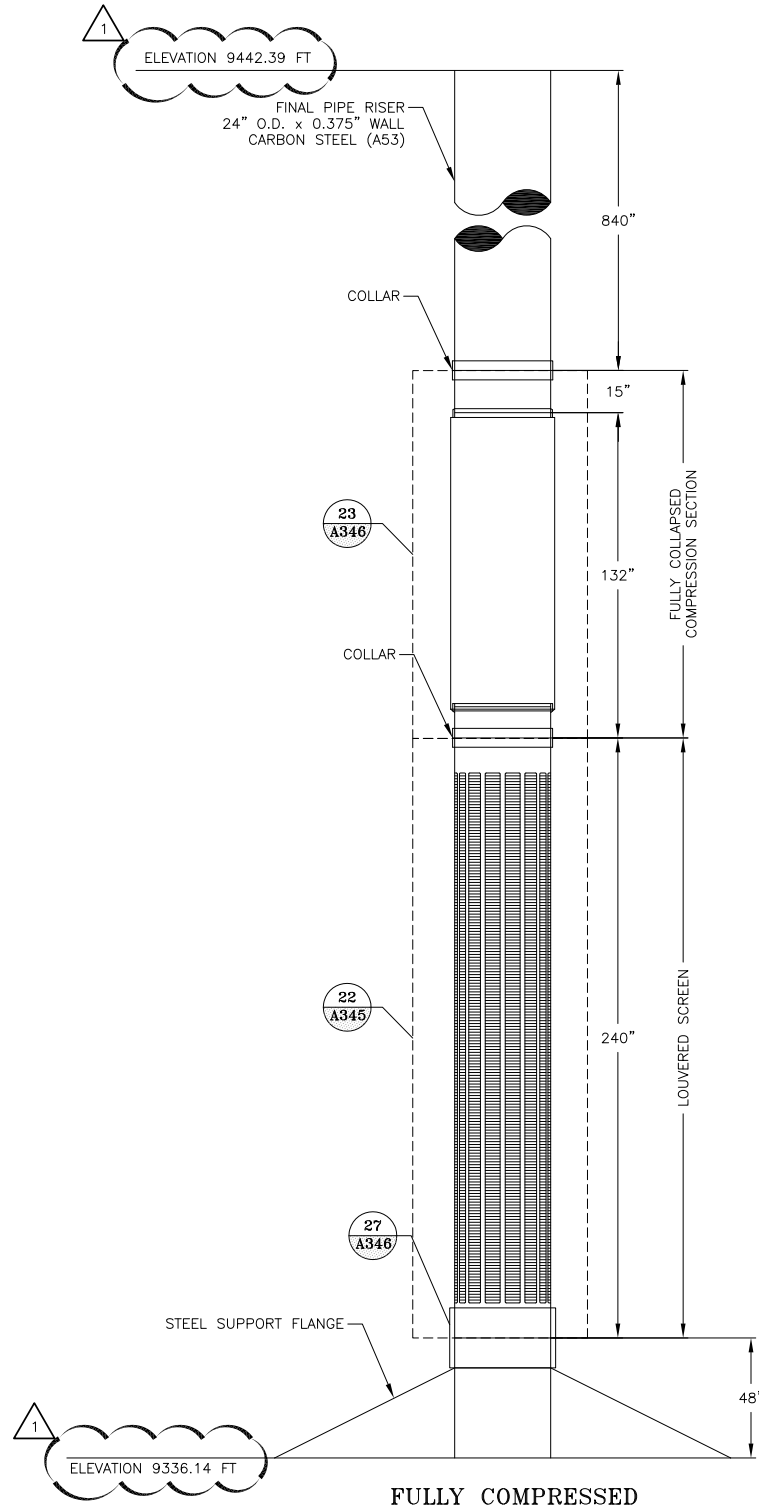
21 HIGH VOLUME SOLUTION COLLECTION SYSTEM VERTICAL RISER DETAIL A330
