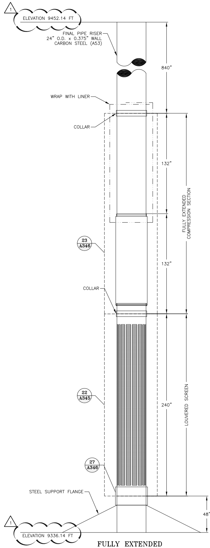
21 HIGH VOLUME SOLUTION COLLECTION SYSTEM VERTICAL RISER DETAIL A330
