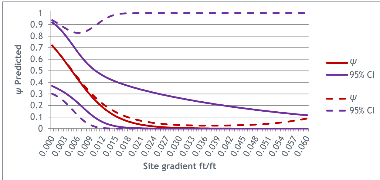
Figure 1.2. Predicted occupancy produced by the top-ranked Flannemouth Sucker model (solid lines) and by model averaging (dashed lines, 30 models) for species-specific historic sites over the range of site gradient potential.
