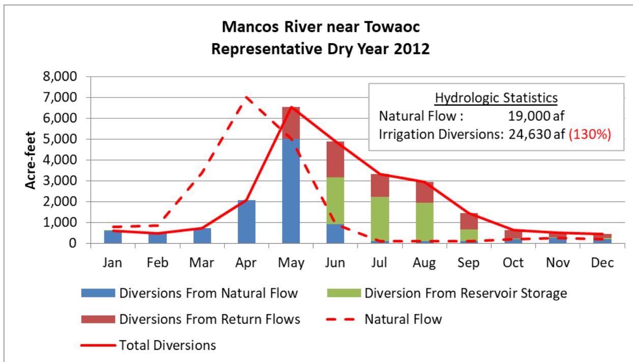
Figure 2-33: Source of Diversion Water for Dry Year 2012
