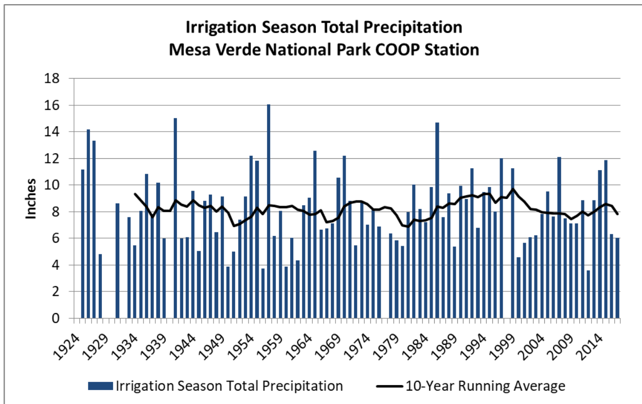
Figure 2-11: Total Irrigation Season Precipitation at Mesa Verde National Park (1924-2017)
