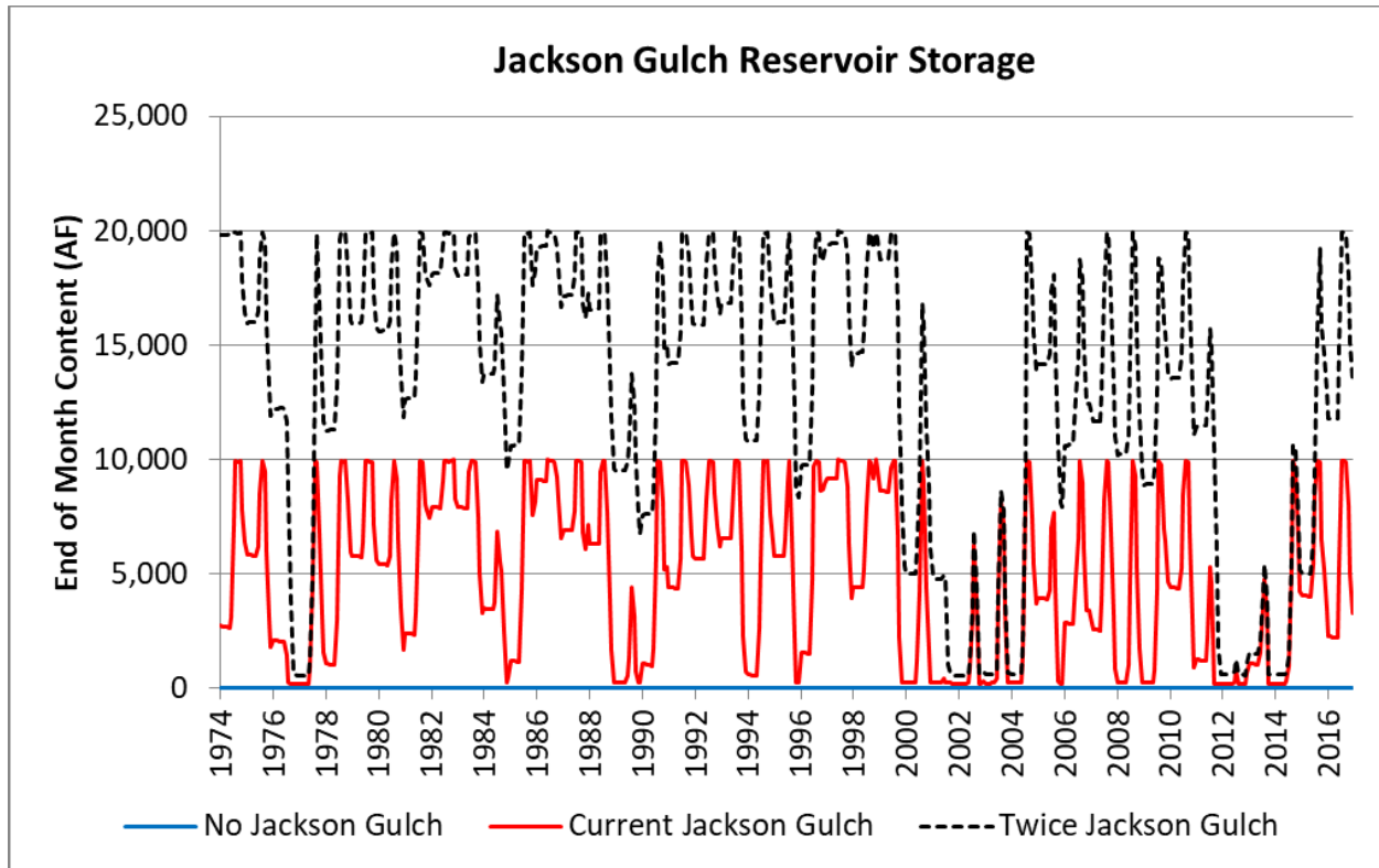
Figure 3-14: Comparing Reservoir Storage Contents from the Jackson Gulch Capacity Scenarios
