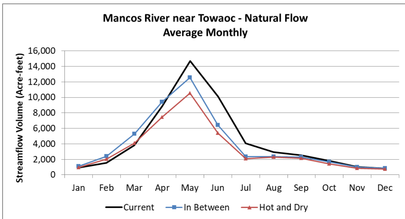
Figure 3-11: Average Monthly Natural Flow at Mancos River near Towaoc under Current Hydrology and Climate Projected Hydrology
