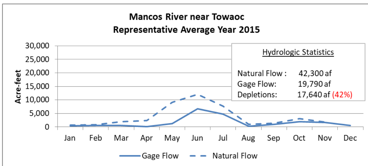
Figure 2-36: Monthly Gage Flow Compared to Natural Flow for Representative Average Year 2015
