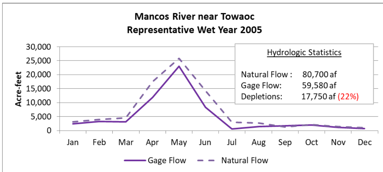
Figure 2-35: Monthly Gage Flow Compared to Natural Flow for Representative Wet Year 2005
