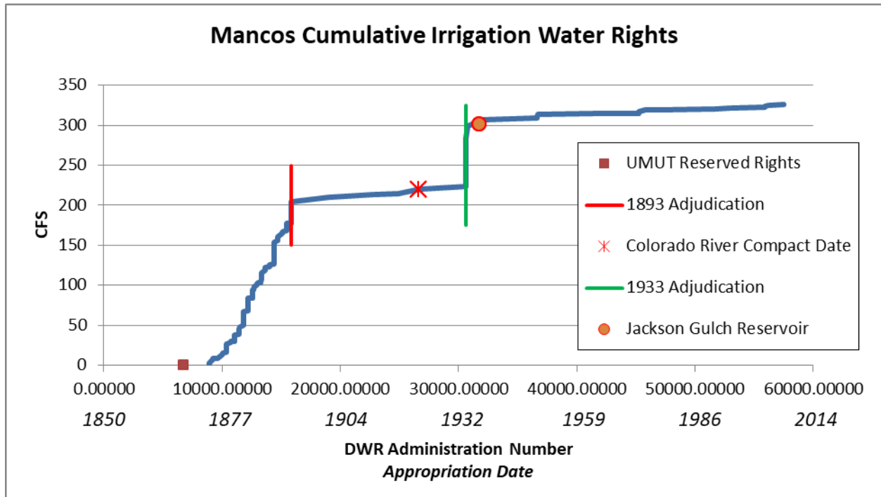
Figure 2-18: Mancos River Valley Cumulative Direct Flow Water Rights
