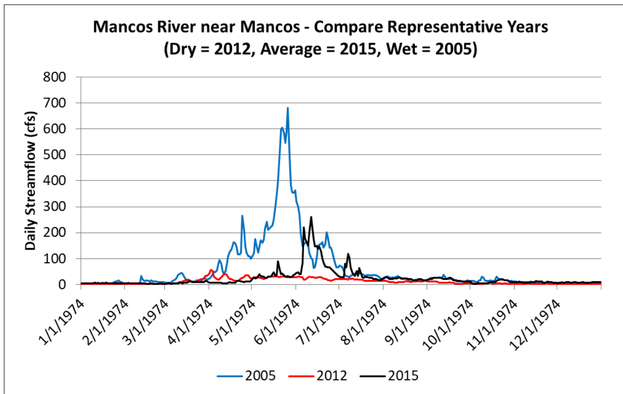
Figure 2-9: Representative Dry, Average, and Wet years for the Mancos River near Mancos
