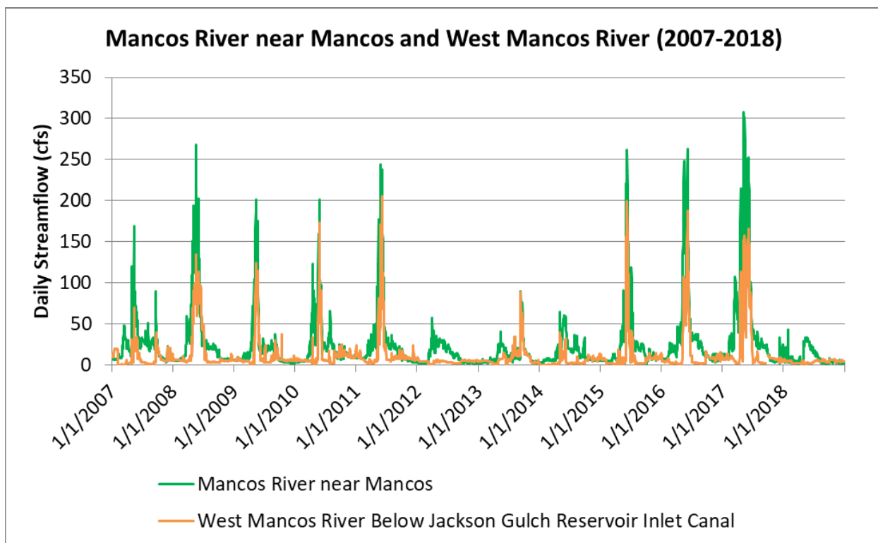
Figure 2-5: Mancos River near Mancos and West Mancos River Streamflow (2007-2018)
