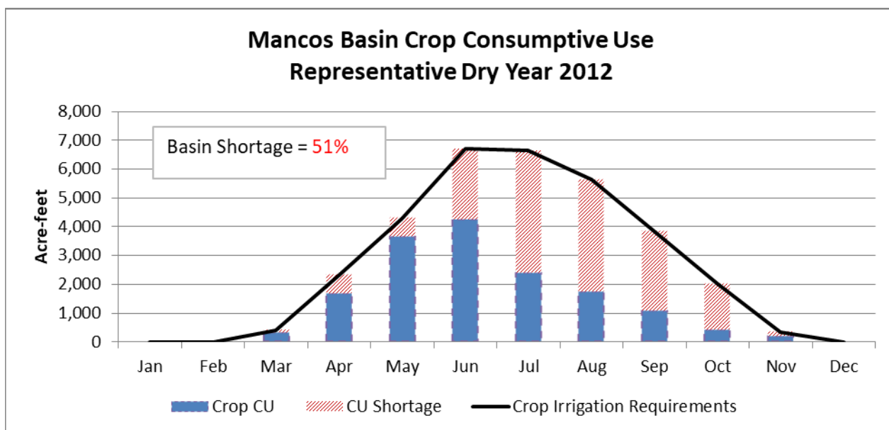
Figure 3-5: Mancos Basin Crop Consumptive Use in Representative Dry Year 2012
