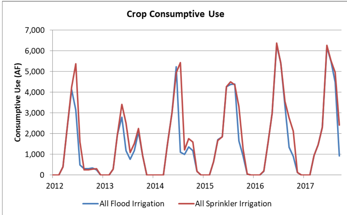
Figure 3-16: Comparing Monthly Crop Consumptive Use for the Irrigation Practices Scenarios
