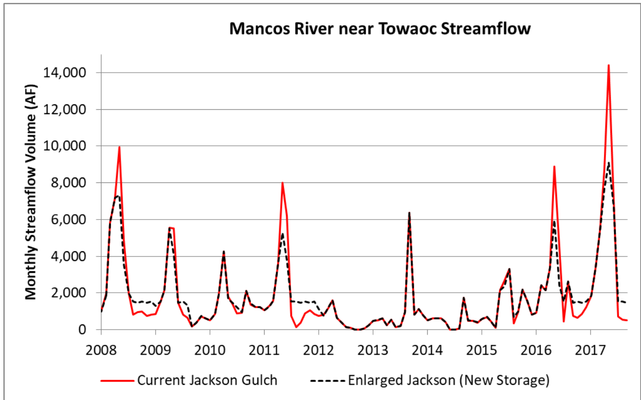
Figure 3-20: Comparing Mancos River near Towaoc Streamflow for the New Storage Scenario
