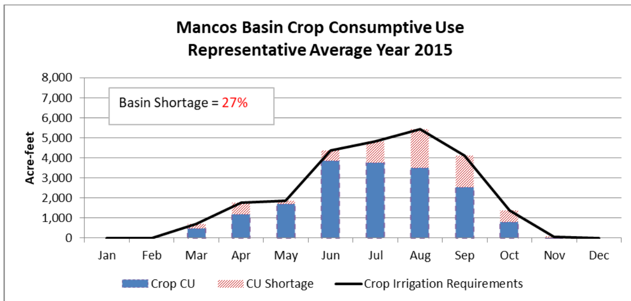
Figure 3-4: Mancos Basin Crop Consumptive Use in Representative Average Year 2015
