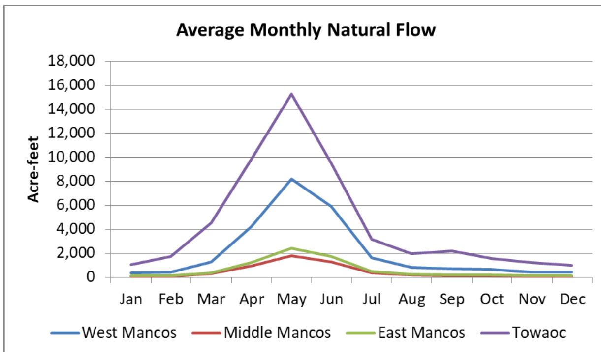
Figure 2-12: Average Monthly Natural Flow at Select Locations in the Mancos Watershed
