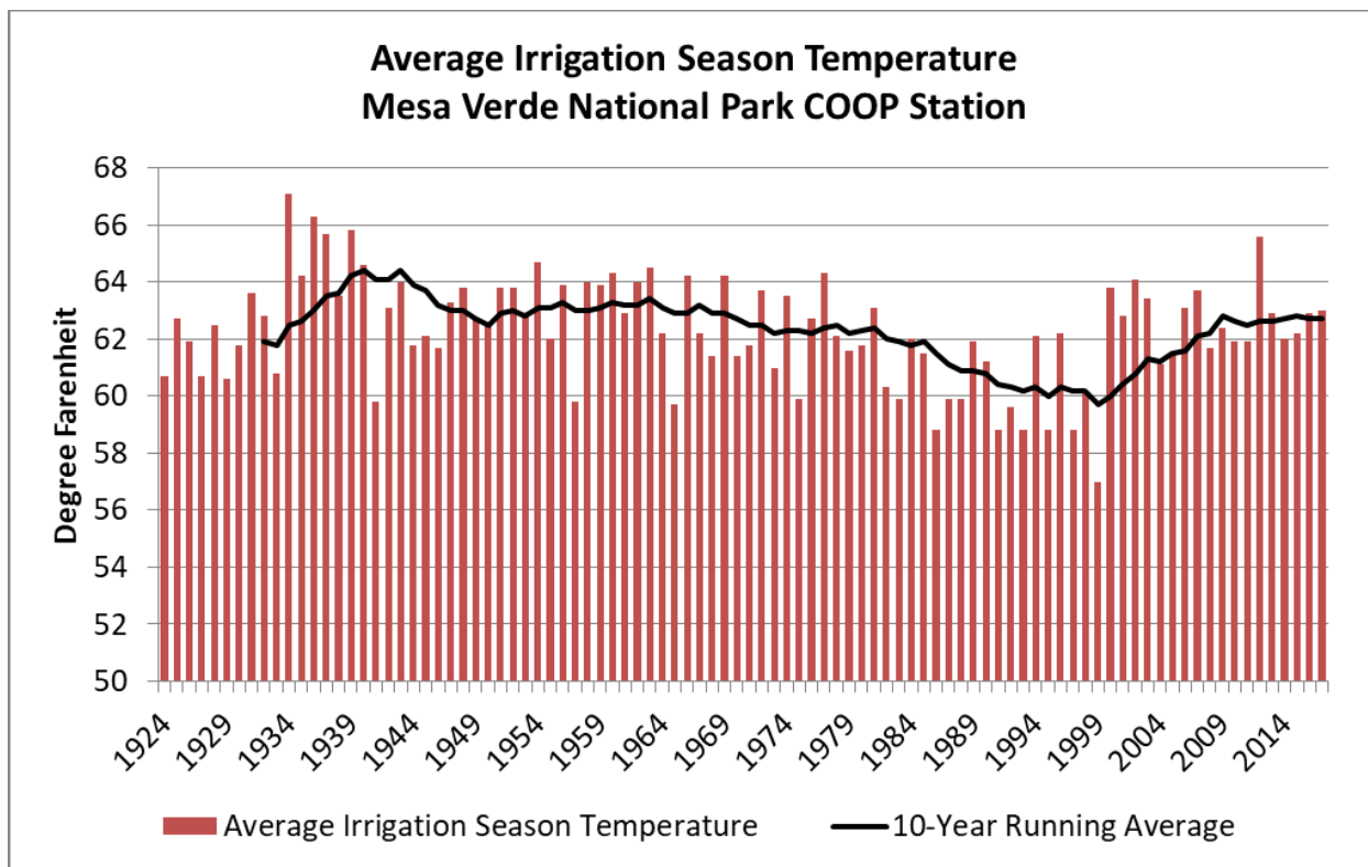
Figure 2-10: Average Irrigation Season Temperature at Mesa Verde National Park (1924 - 2017)
