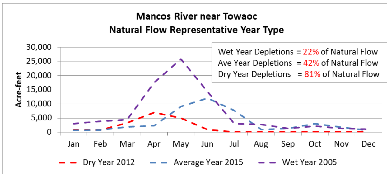
Figure 2-38: Monthly Natural Flow Compared for Three Representative Years (2005, 2012, and 2015)
