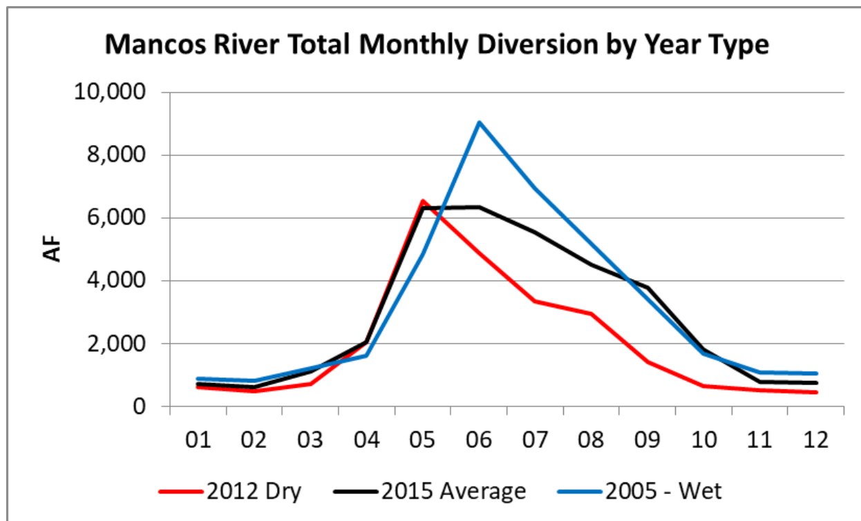
Figure 2-16: Mancos Valley Total Monthly Diversions for Irrigation by Year Type
