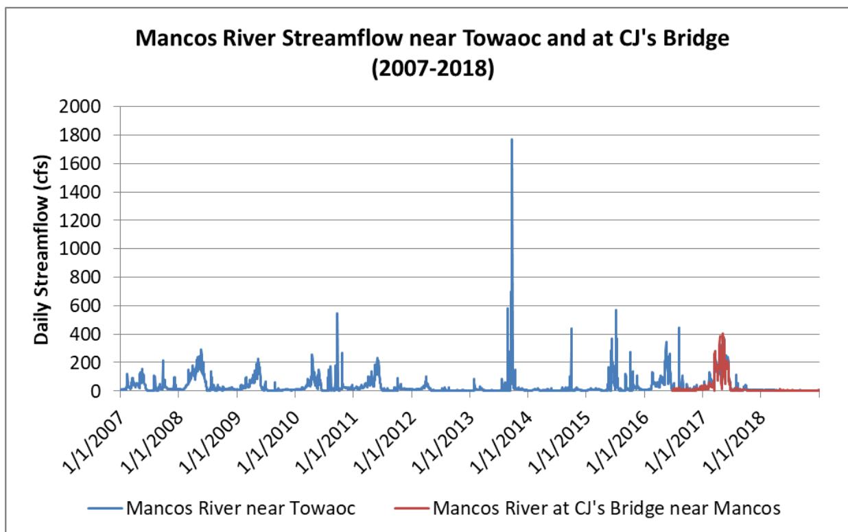
Figure 2-3: Mancos River Streamflow near Towaoc and at CJ's Bridge (2007-2018)
