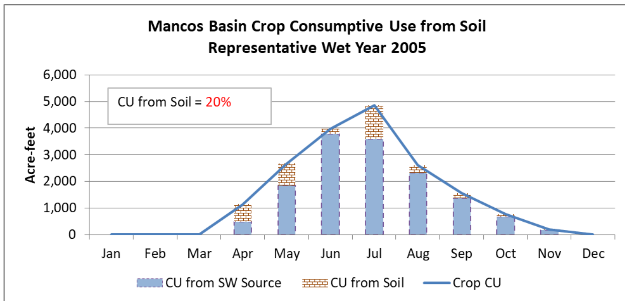
Figure 3-7: Mancos Basin Crop Consumptive Use from Soil Moisture for Representative Wet Year 2005
