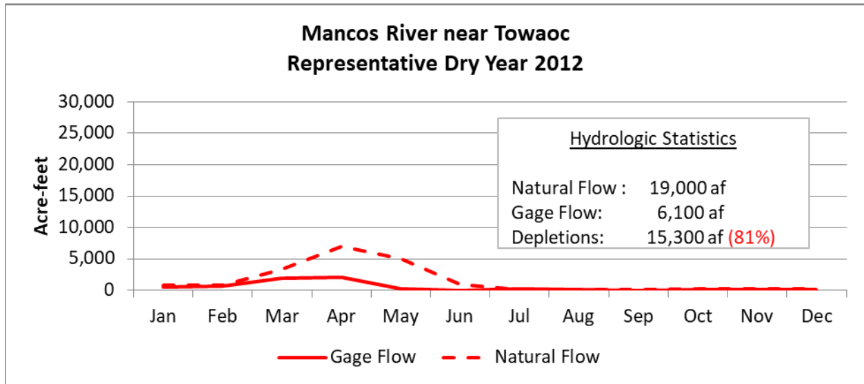
Figure 2-37: Monthly Gage Flow Compared to Natural Flow for Representative Dry Year 2012
