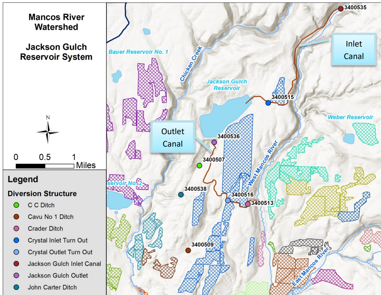
Figure 2-22: Jackson Gulch Reservoir and Related Infrastructure
