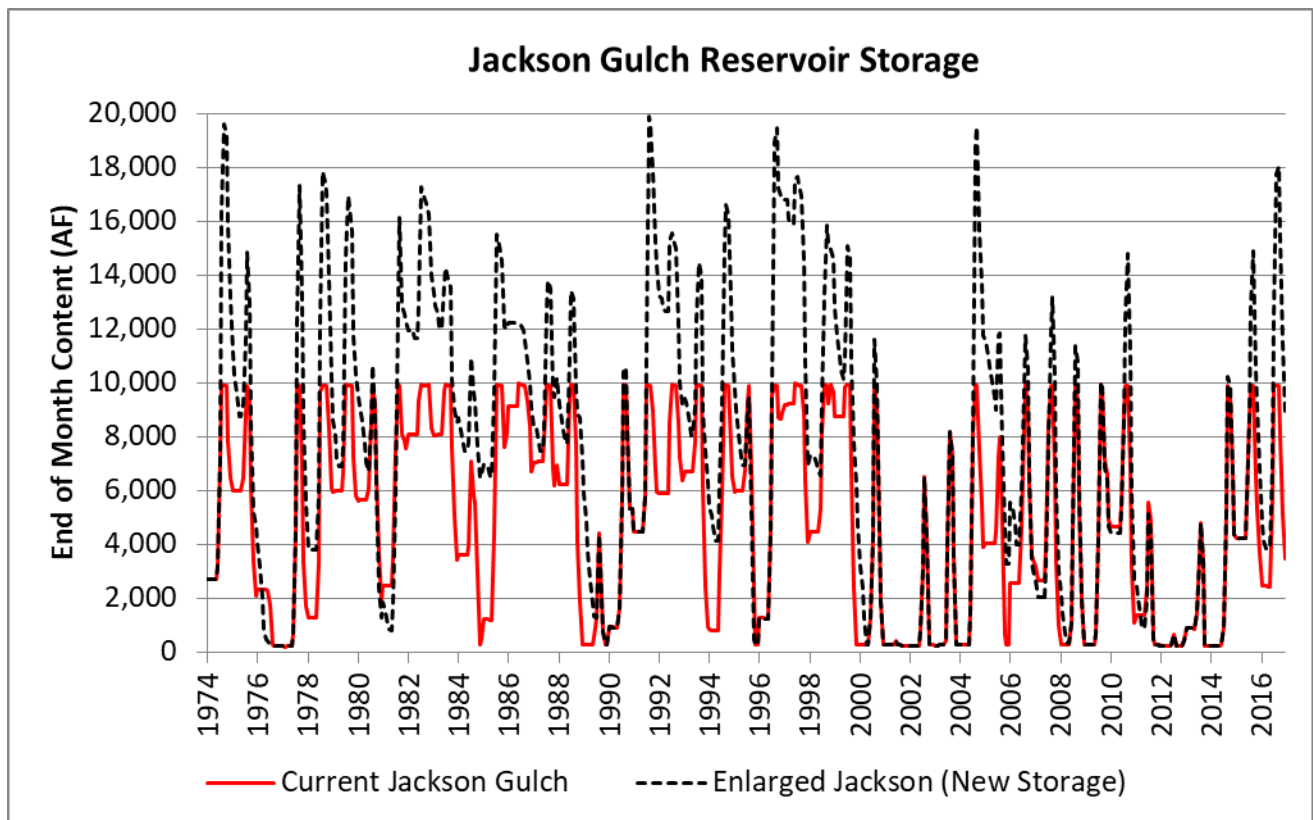
Figure 3-19: Comparing Jackson Gulch Reservoir Storage for the New Storage Scenario
