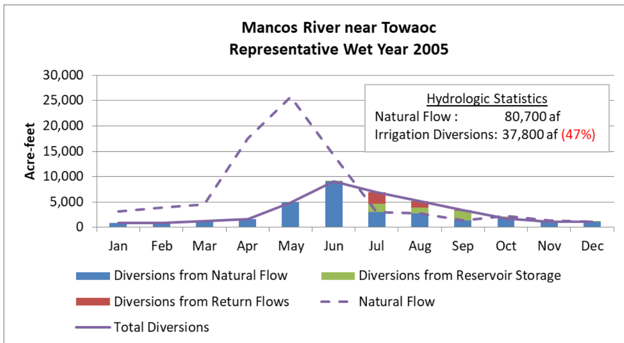
Figure 2-31: Source of Diversion Water for Wet Year 2005
