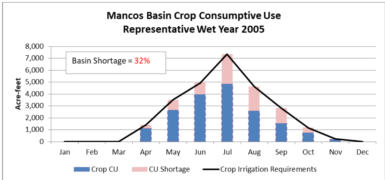
Figure 3-3: Mancos Basin Crop Consumptive Use in Representative Wet Year 2005
