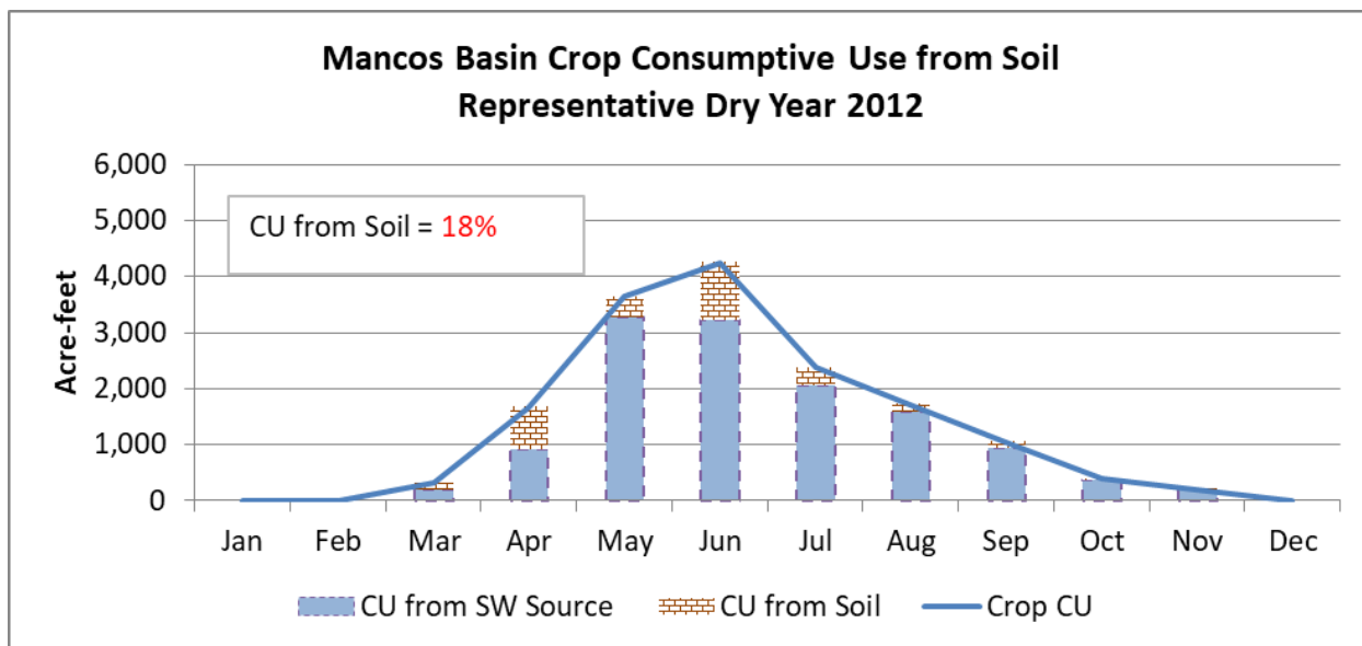
Figure 3-8: Mancos Basin Crop Consumptive Use from Soil Moisture for Representative Dry Year 2012
