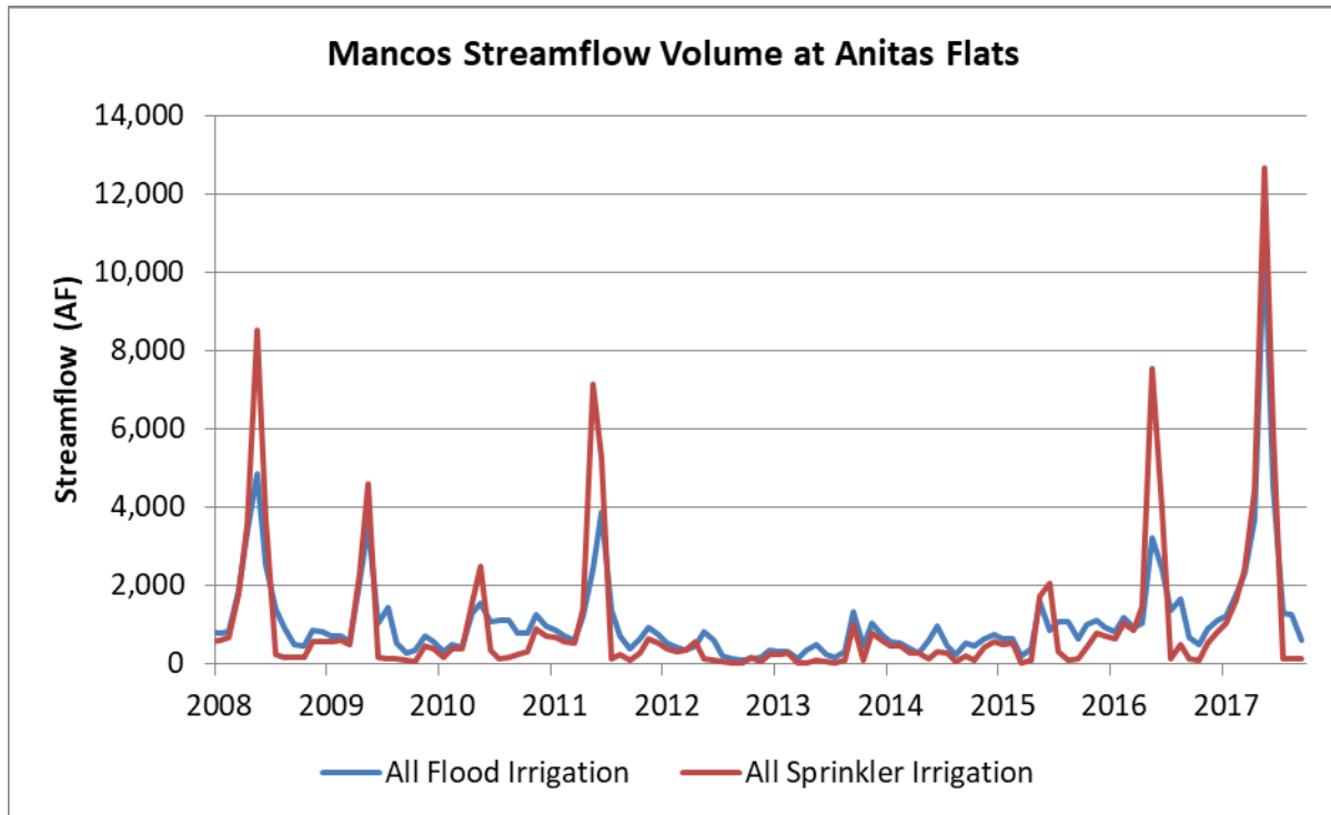
Figure 3-18: Comparing Monthly Mancos River Streamflow for the Irrigation Practices Scenarios
