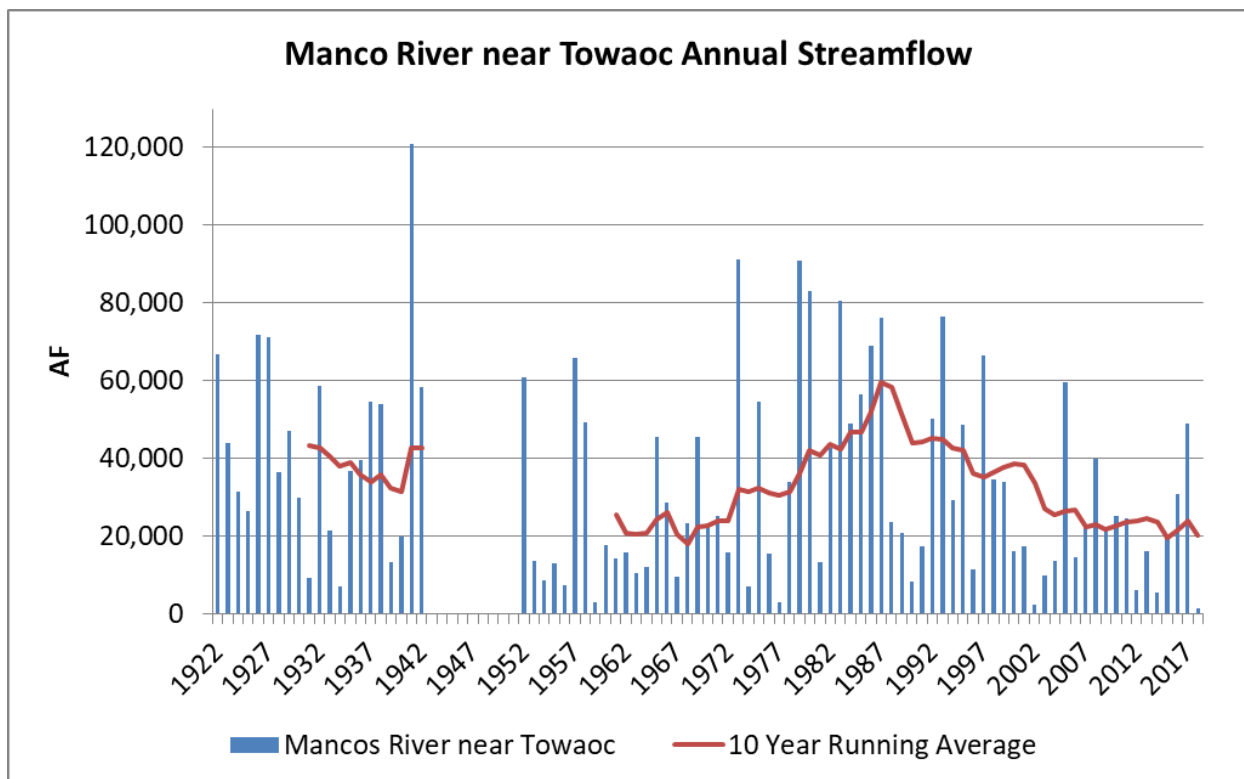
Figure 2-6: Mancos River near Towaoc Annual Streamflow Volume (1922 - 2018) (acre-feet)
