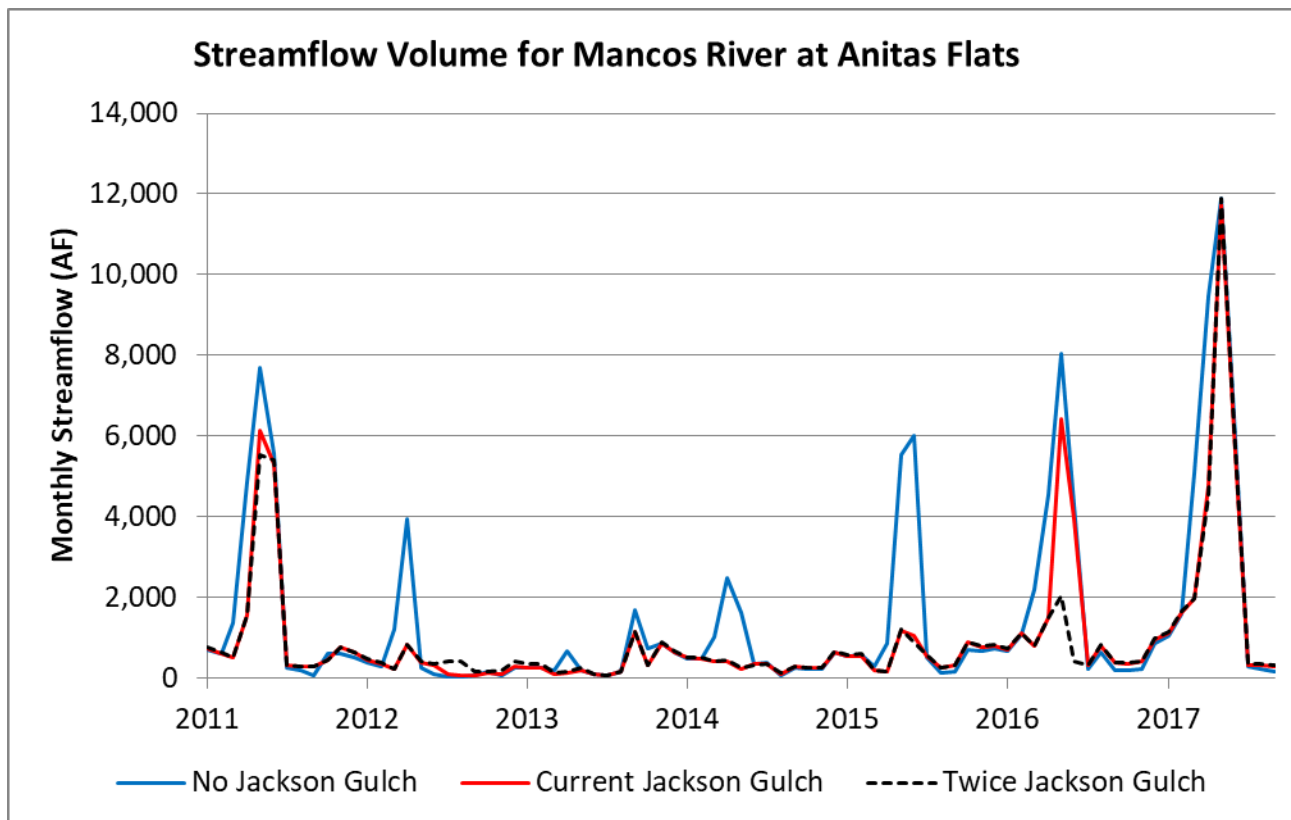
Figure 3-15: Comparing Monthly Streamflow Volume for Jackson Gulch Reservoir Capacity Scenarios
