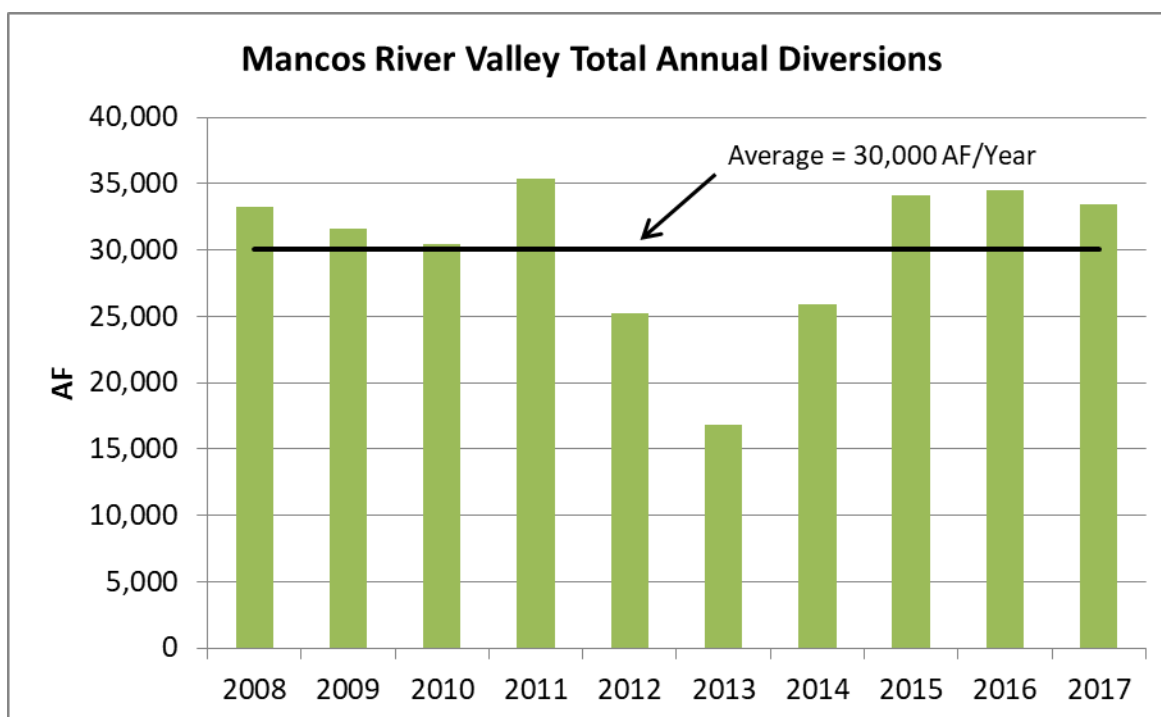
Figure 2-15: Annual Mancos River Valley Diversions
