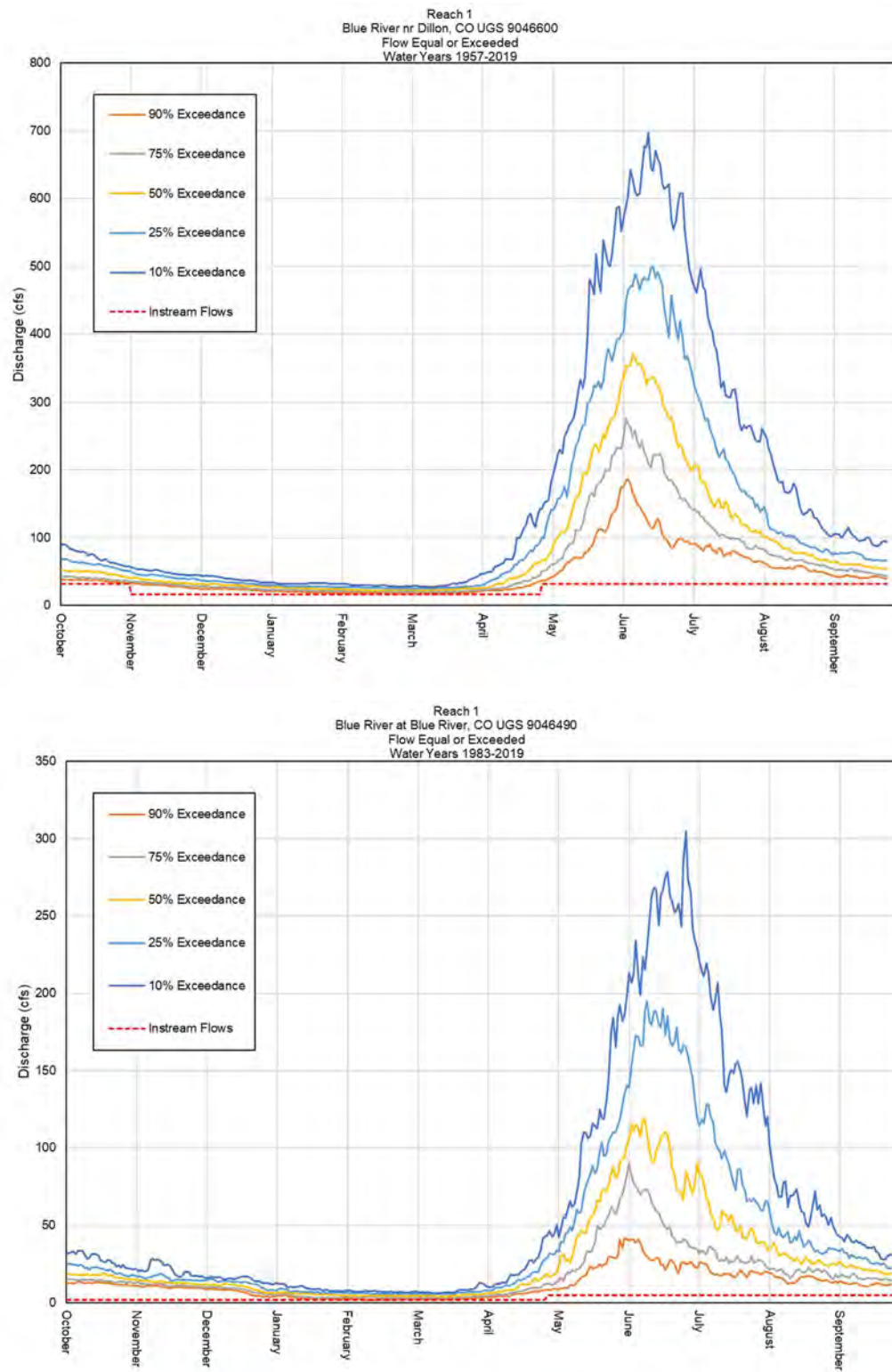
Figure B-4. Exceedance Plots for the Four Blue River Main Stem Gage Sites (cont.).
