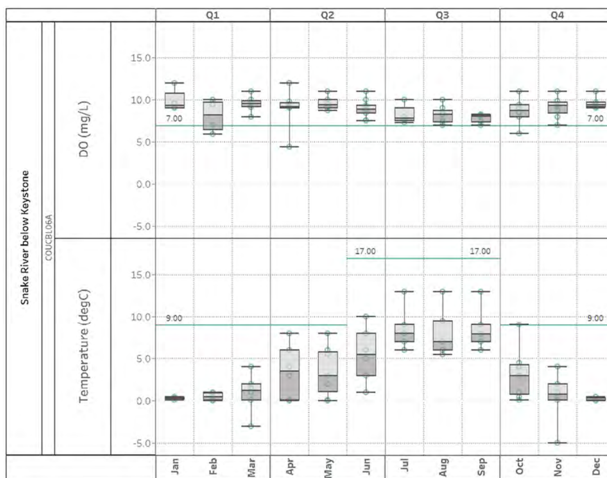
Figure C9 DO (mg/L) and Temperature ( ^{\circ}\text{C} ) values at Snake River below Keystone. The color denotes the sites Regulation No. 33 segment ID. Relevant water quality standards are also overlaid in the plot. The box & whisker diagrams in the plot highlight statistics of the dataset. The box spans the 25th to 75th percentile and the median is shown as a dark bar in the box. The whiskers extend to the minimum and maximum values in the dataset.
