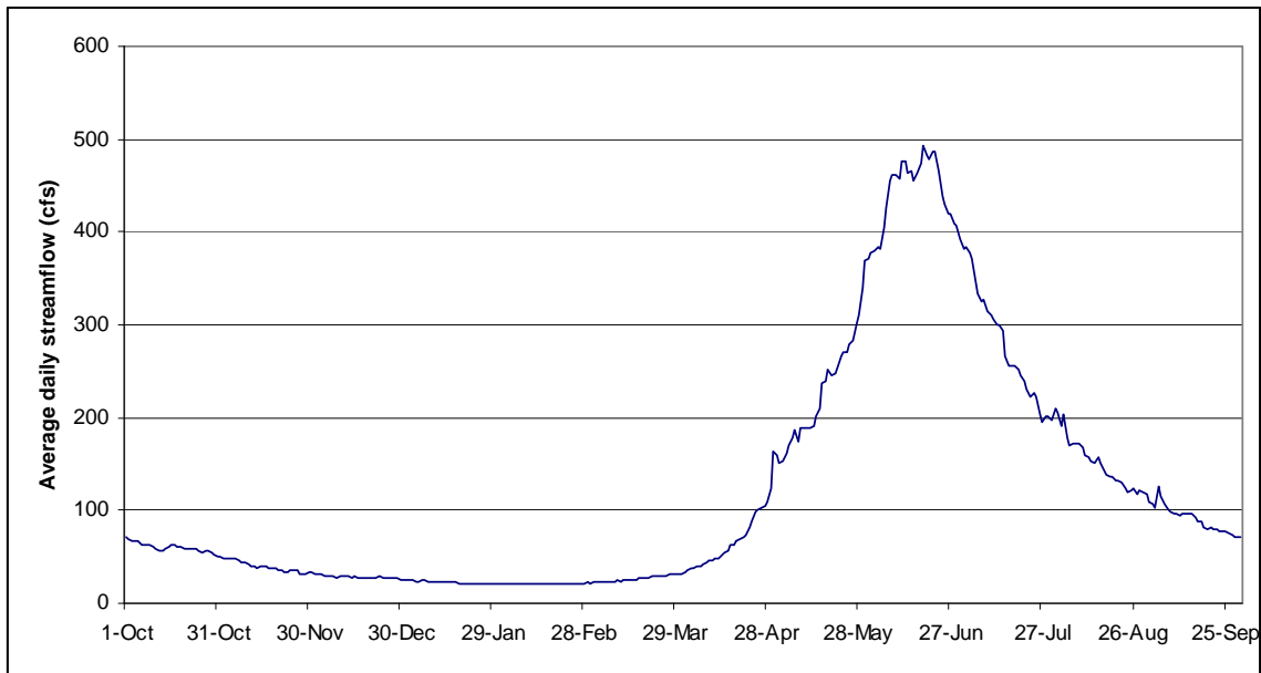
Figure 23. Big Thompson River at Mouth of Canyon, USGS (0673800) historical gage flows (1927-2004).
