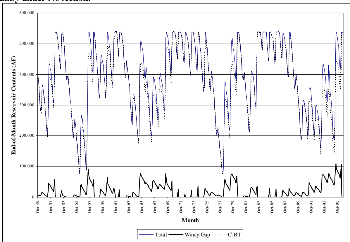
Figure 29. End-of-Month Storage Volume of C-BT and Windy Gap Water in Lake Granby under No Action.
