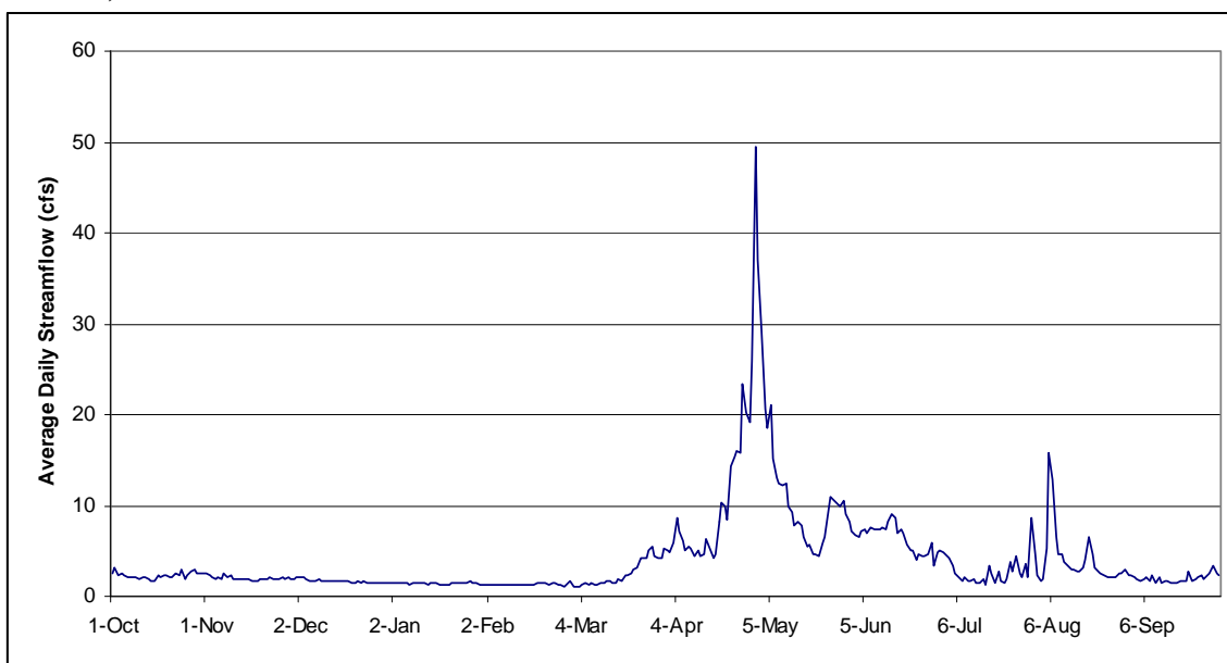
Figure 17. Coal Creek near Louisville, USGS (06730400) historical gage flows (1997-2004).
