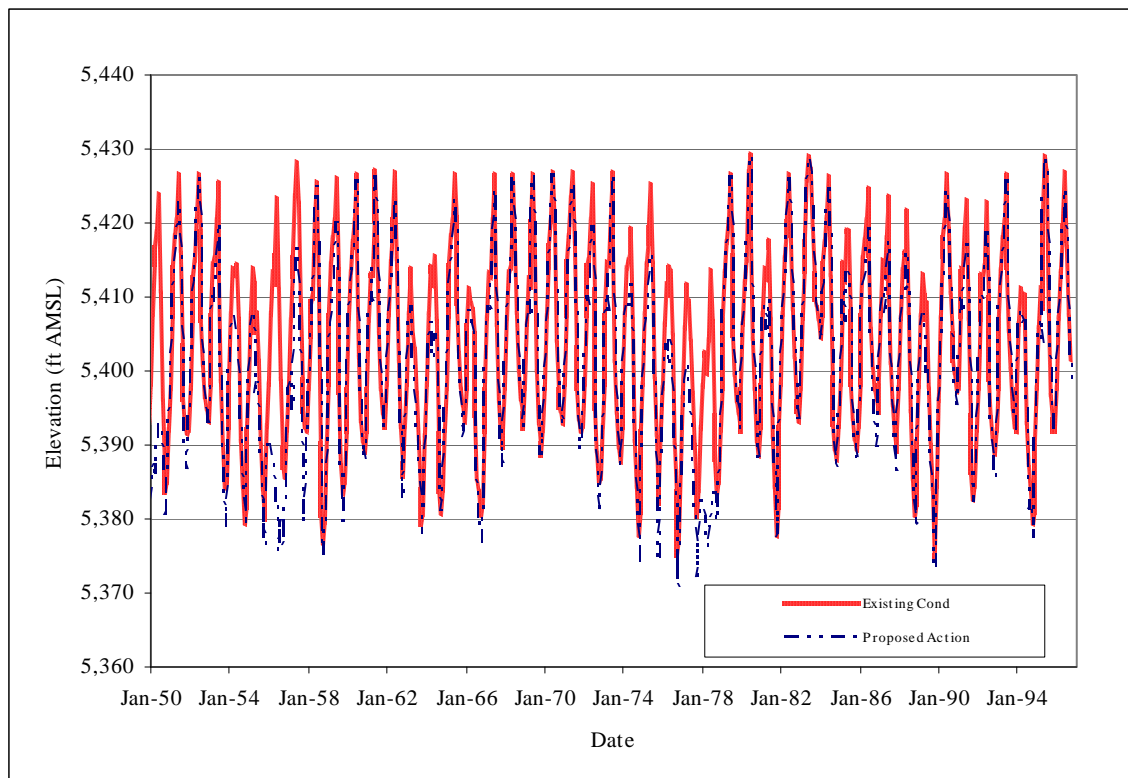
Figure 41. Horsetooth Reservoir estimated average monthly surface elevation for the Proposed Action.
