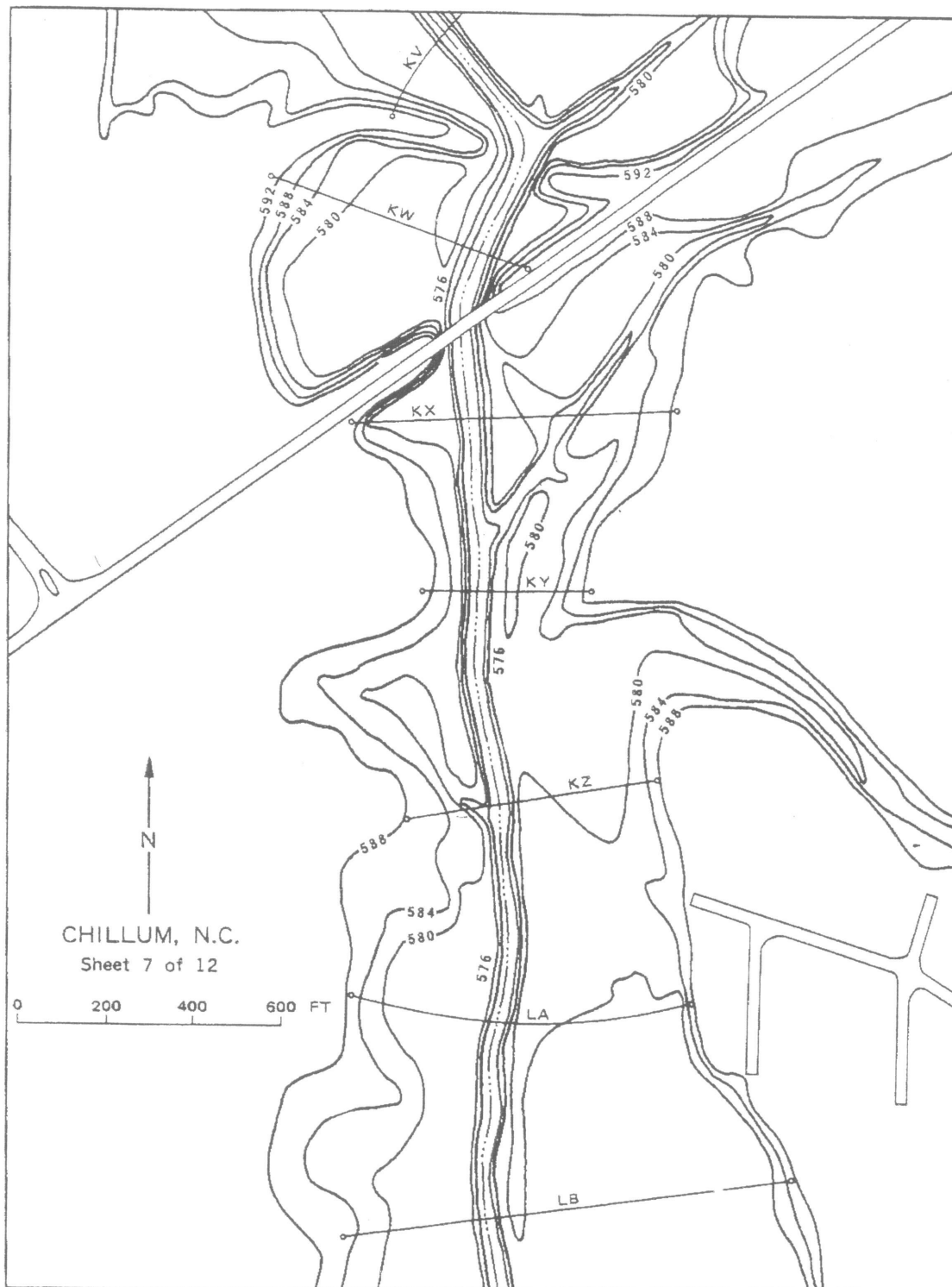
Figure A-3. Example Floodplain Contours
