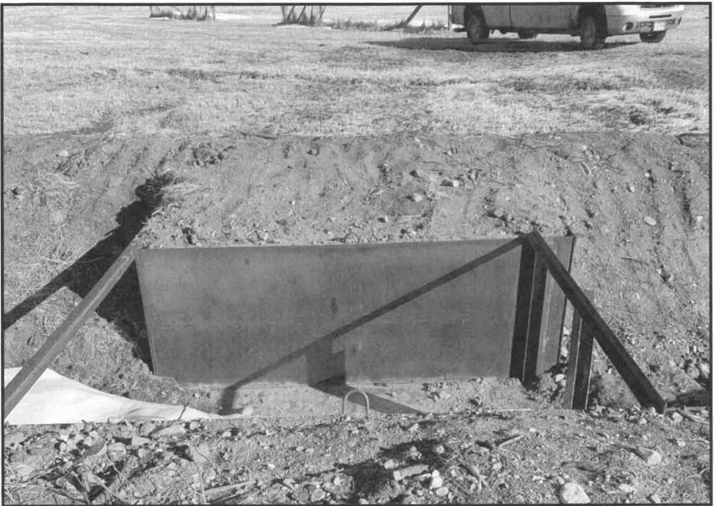
Photos of backfilled structure. 1/4" steel walls and floor with 1/4" x 2" x 2" angle iron reinforcement and check board slots. Dimensions and elevations are as designed. Welds and construction are good. Compaction is present and installation is good. Anodes are in place - (2) 32lb.
