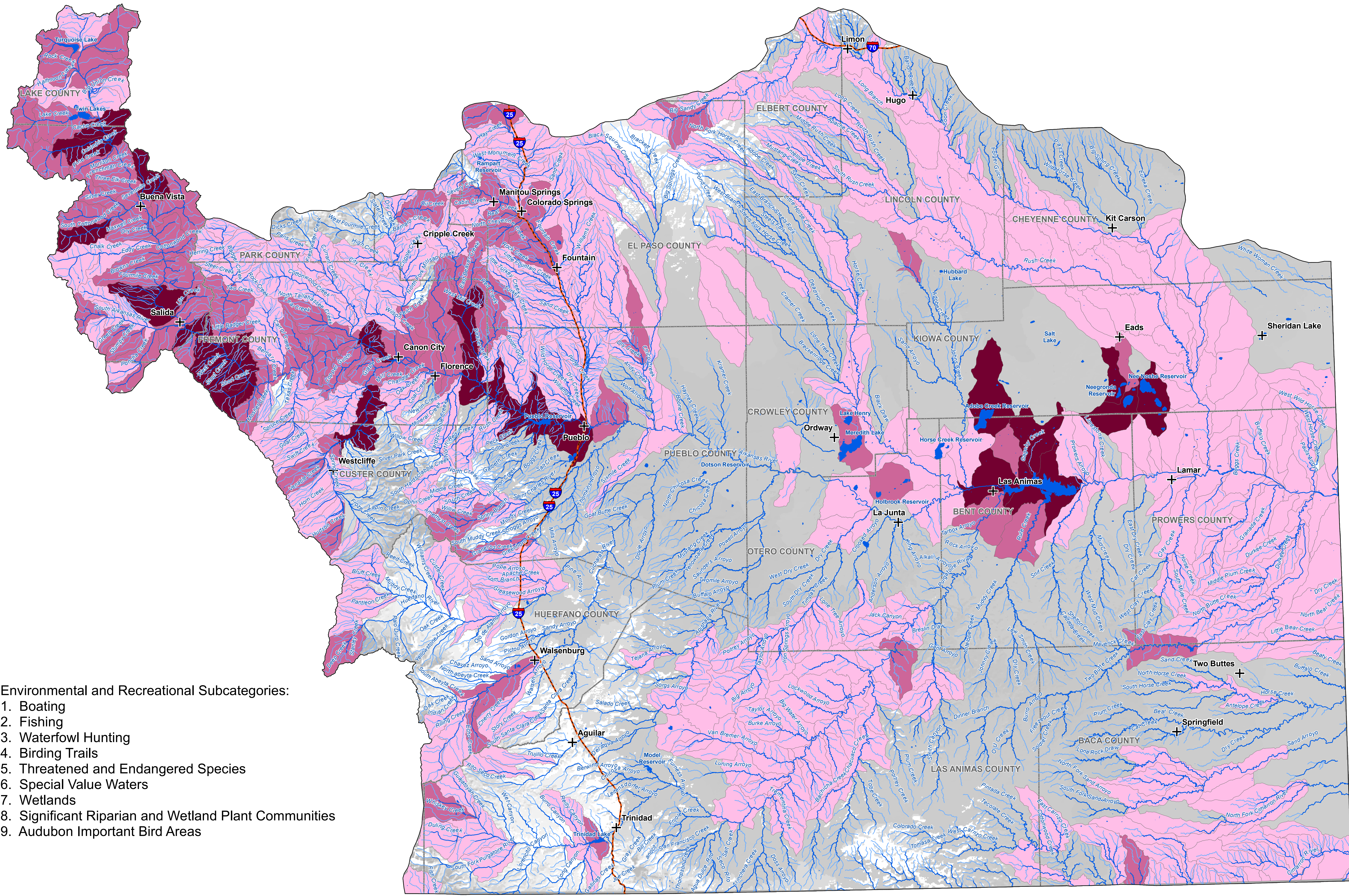
Figure 2-6 Arkansas Basin Nonconsumptive Needs Assessment Environmental and Recreational Subcategories by 12-Digit HUC
