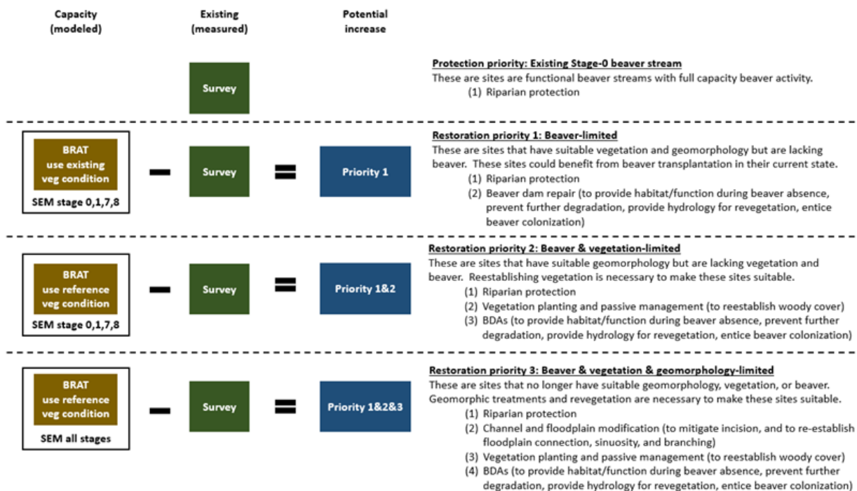
Figure 1. Schematic showing how this study quantifies the potential for beaver restoration. Basin-wide beaver activity surveys (pond area/mile, dams/mile) define the existing level. Capacity is predicted using BRAT, and the potential for increase is the difference of capacity minus existing. Reaches with a high level of beaver activity are protection priorities. Restoration priorities 1-3 represent reaches for which increasing levels of effort are required to restore sustainable beaver activity. Capacity for the priority 1 (beaver-limited) condition is given by BRAT simulations using existing vegetation on reaches that are not entrenched. Increased capacity for the priority 2 (beaver & vegetation-limited) condition is estimated by BRAT simulations that use reference vegetation on reaches that are not entrenched, assuming that vegetation can be restored. Increased capacity for the priority 3 (beaver & vegetation & geomorphology-limited) condition is estimated by BRAT simulations that use reference vegetation on all reaches that are not entrenched, assuming that vegetation and entrenchment can be restored.
