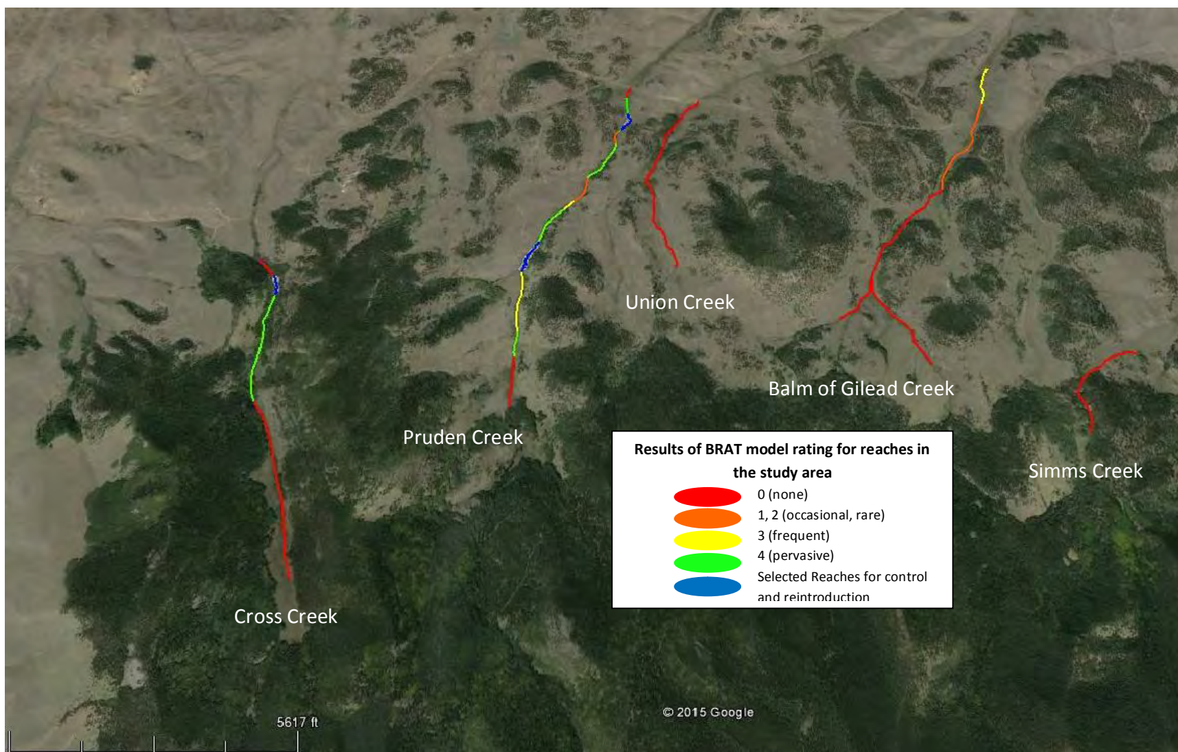
Figure 1: Results of the BRAT model, by reach.
