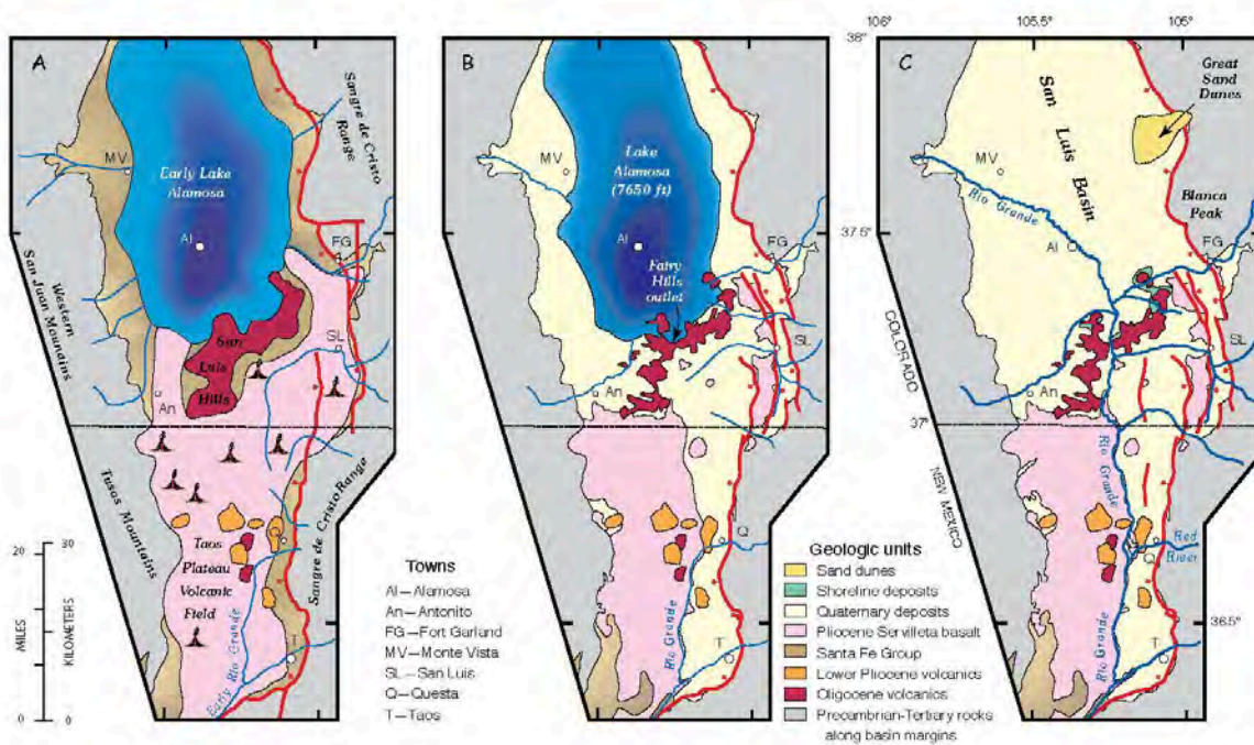
Figure 5.5. Simplified geological map of the San Luis Basin showing generalized geology and drainage patterns for the time intervals, A) 3.5-5 million years before present (BP), B) 4440,000 years BP, and C) Current (taken from Machette et al 2007)..
