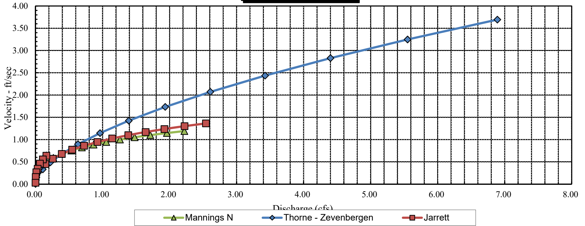
Miners Creek Velocity vs. Discharge
