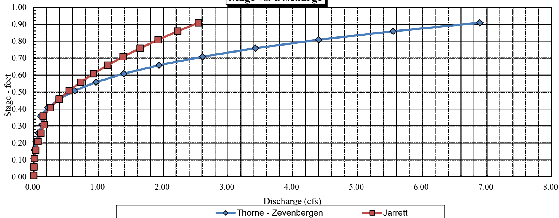
Miners Creek Stage vs. Discharge
