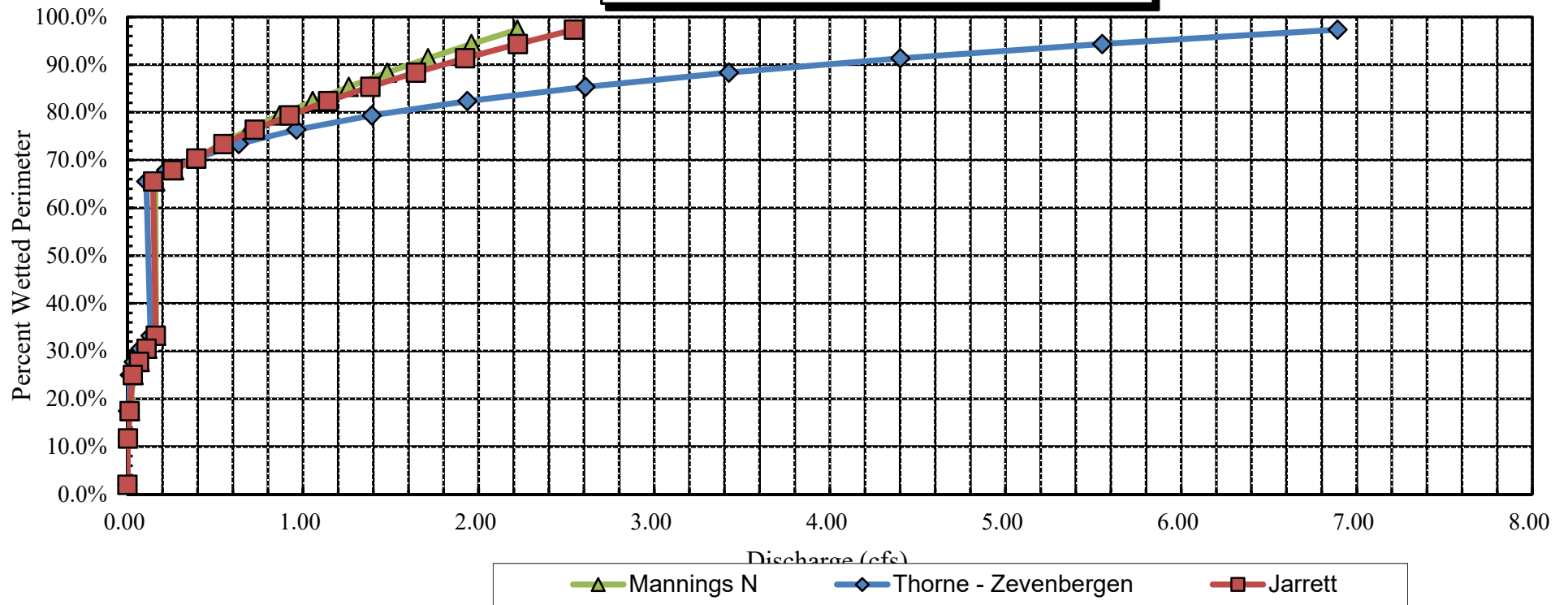
Miners Creek Percent Wetted Perimeter vs. Discharge
