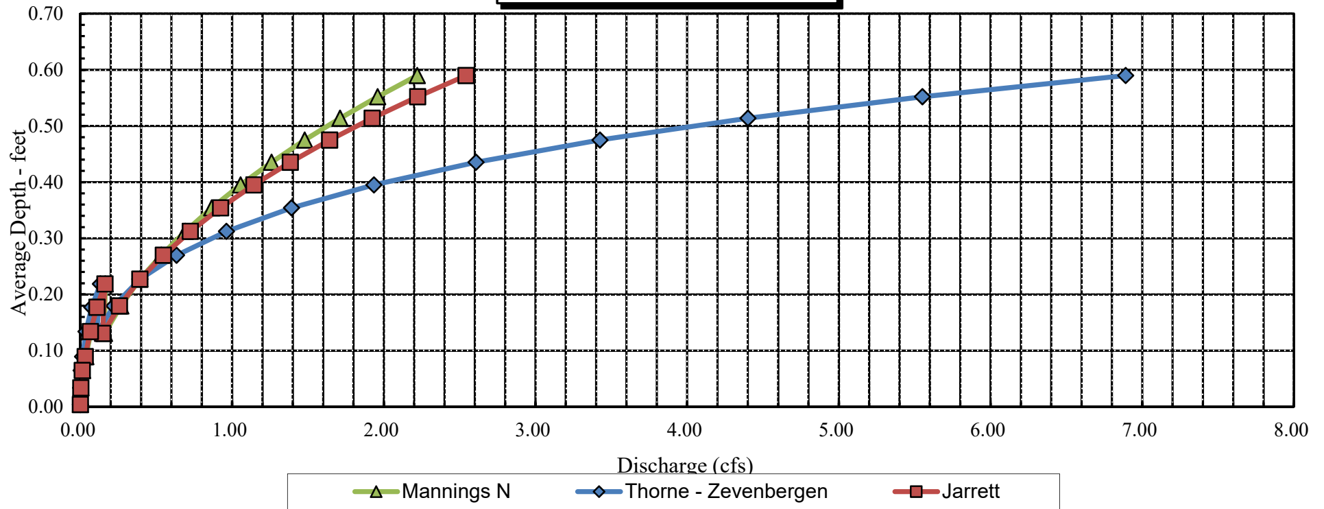
Miners Creek Average Depth vs. Discharge
